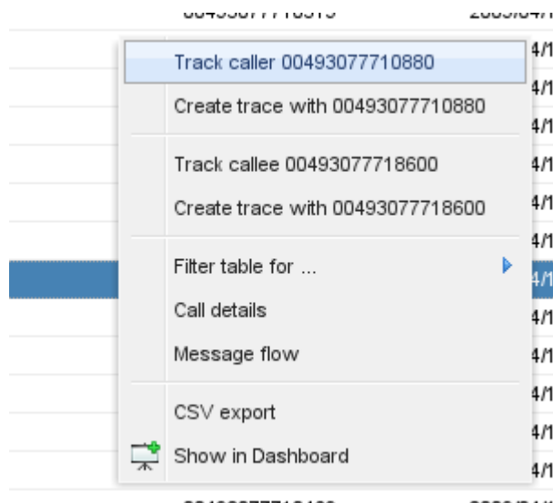
Figure 3–7 Right-Click Menu
