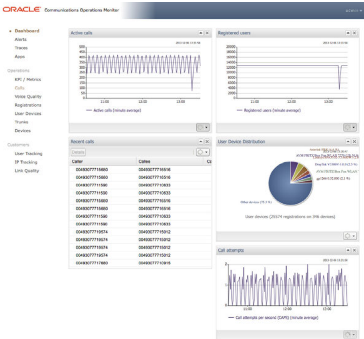
Figure 3–11 Dashboard
