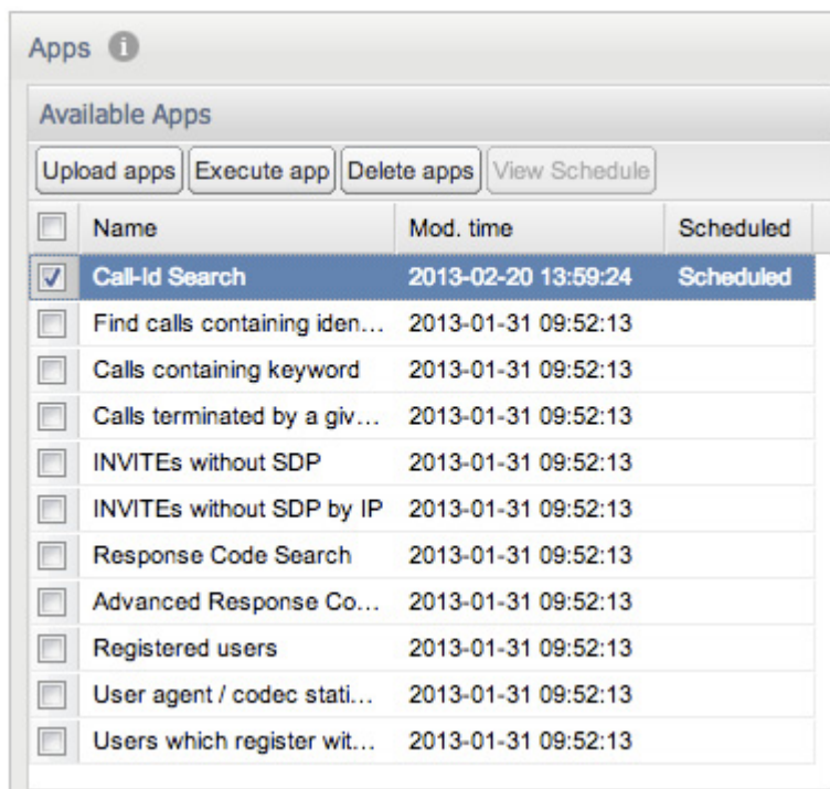
Figure 3–35 Scheduled App
