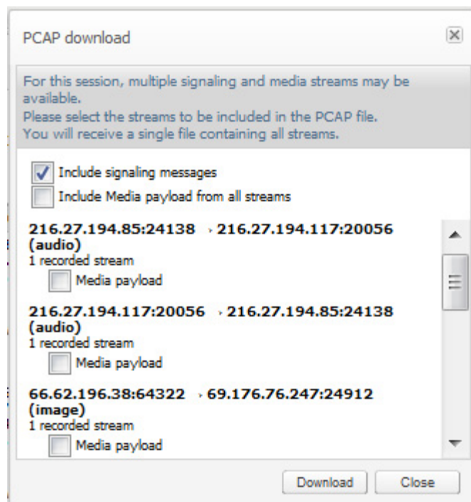
Figure 4–44 Download the Signaling and Recorded Media Streams
