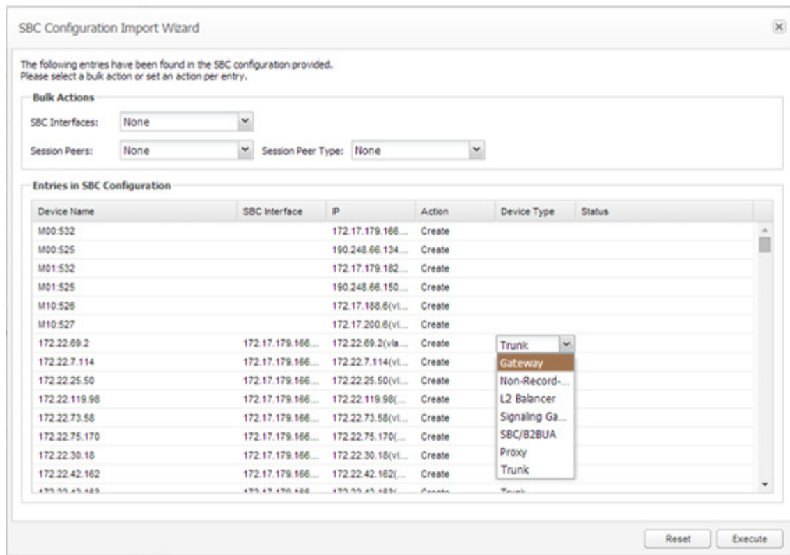
Figure 7–29 SBC Configuration Import Wizard Page
