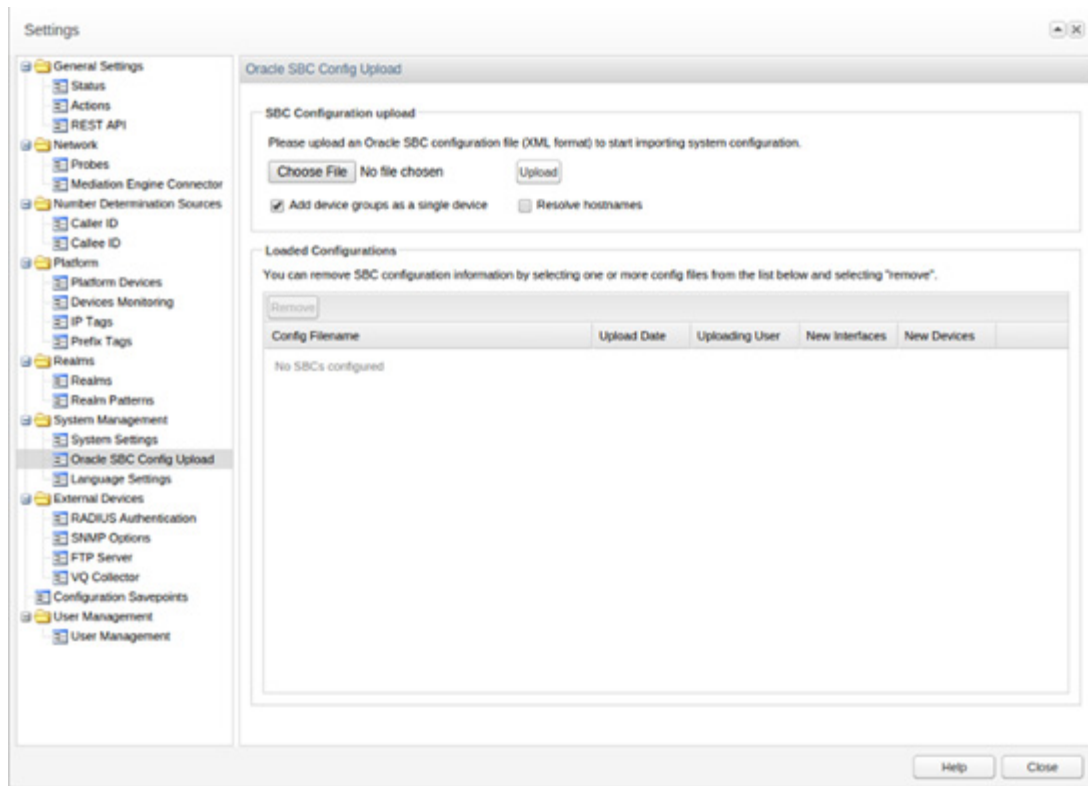
Figure 7–28 Oracle SBC Config Upload Page
