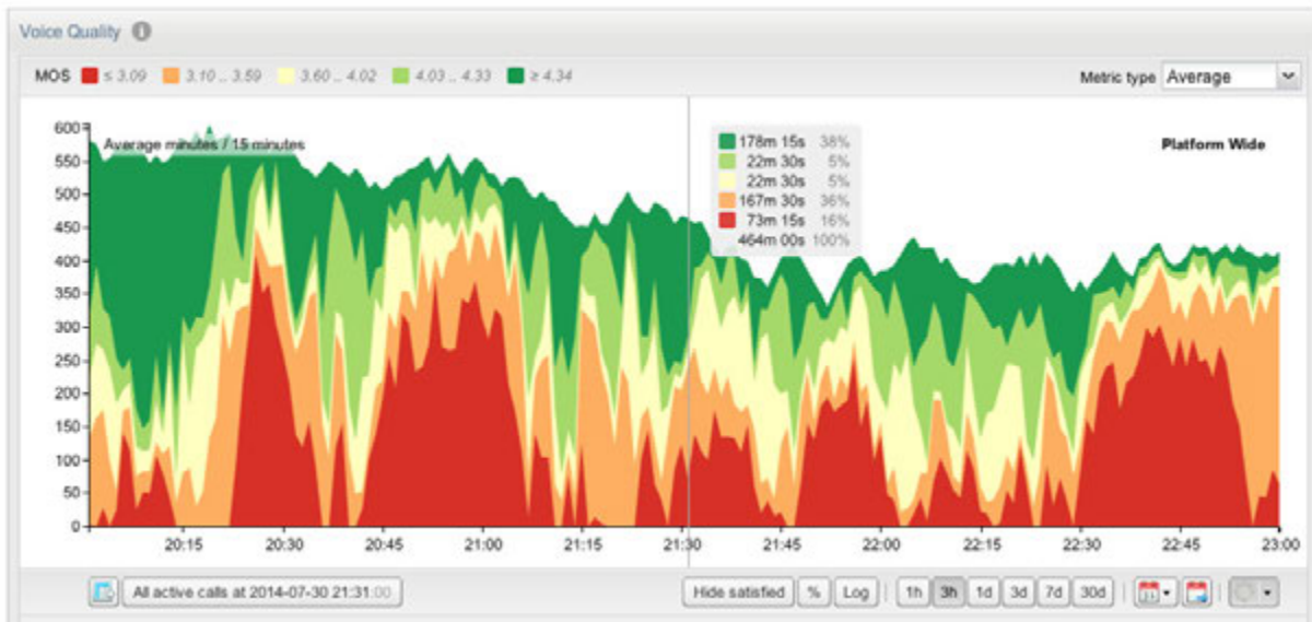
Figure 4–38 Voice Quality Overview
