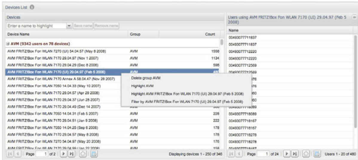
Figure 4–53 Right-Click Menu
