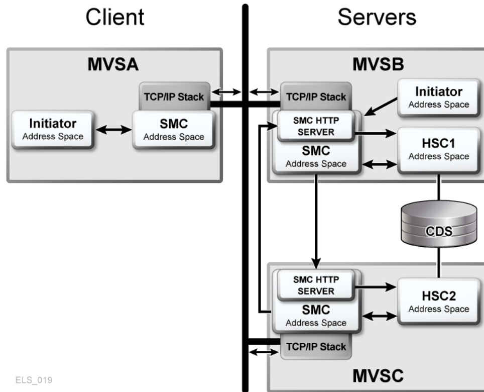
Figure 3–2 Single TapePlex using the SMC Client/Server Feature
