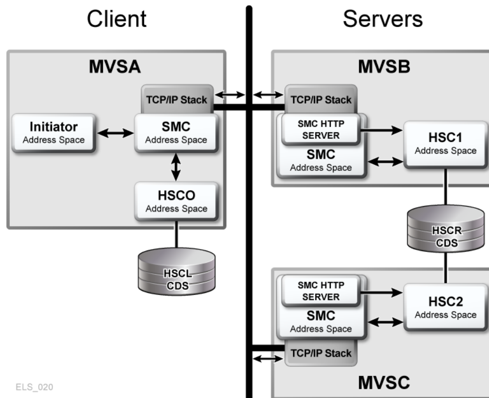
Figure 3-3 Two TapePlexes Accessed by a Single SMC
