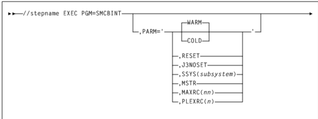
Figure 2-1 SMC EXEC Statement syntax
