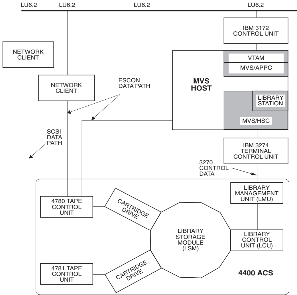
FIGURE 2-2 Typical LibraryStation Configuration for LU6.2 Clients
