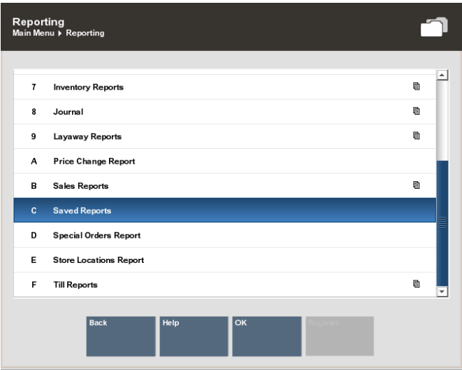
Figure 2–26 Reporting Menu
