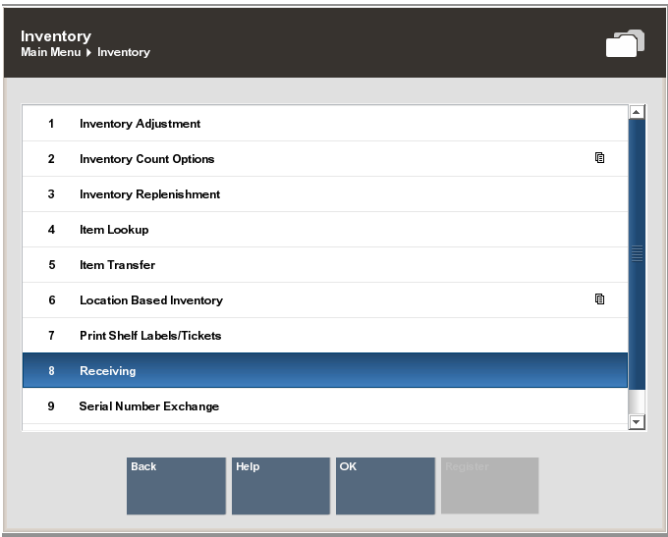
Figure 2–2 Inventory Menu
