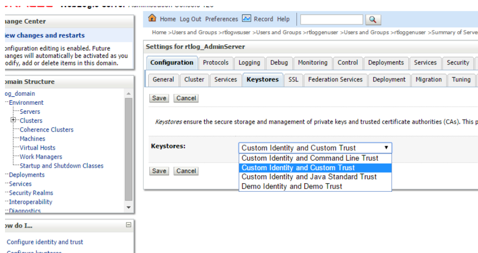
Figure 6–37 Keystores Settings
