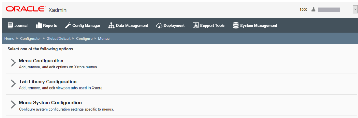
Figure 5–10 Menu Options
