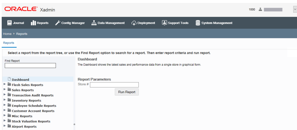
Figure 9–2 Reports - Dashboard
