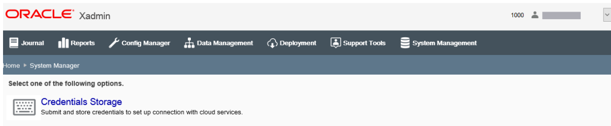
Figure 3–2 System Manager
