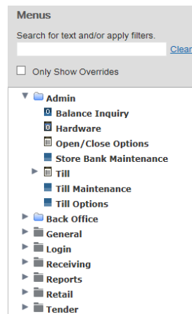
Figure 5–11 Menu Categories
