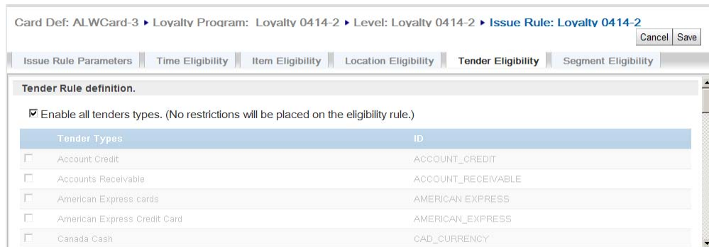
Figure 14-19: Tender Eligibility Tab
