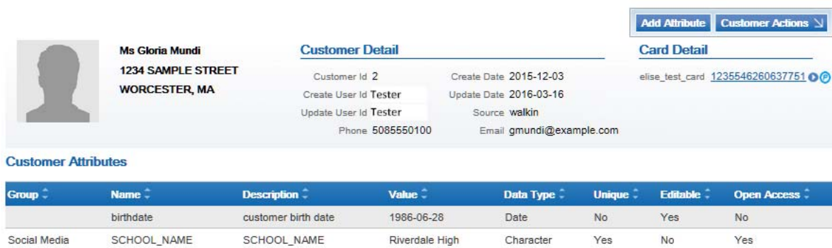
Figure 2-32: Attributes Screen
