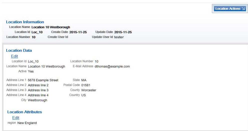
Figure 16-4: Location Dashboard
