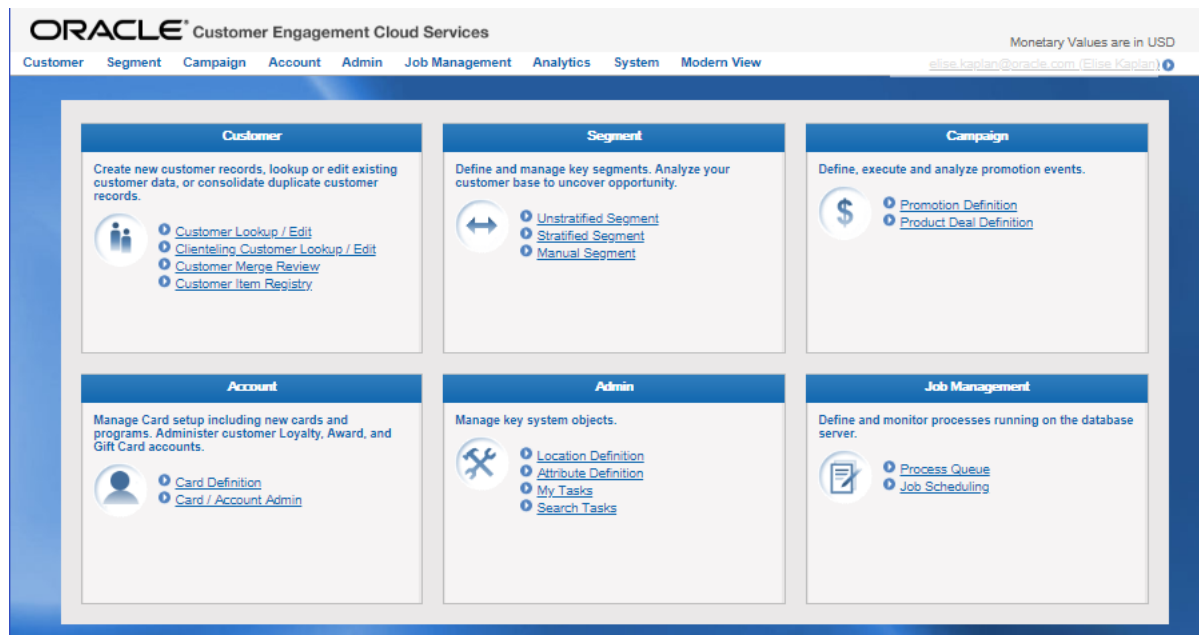
Figure 1-8: Main Page
