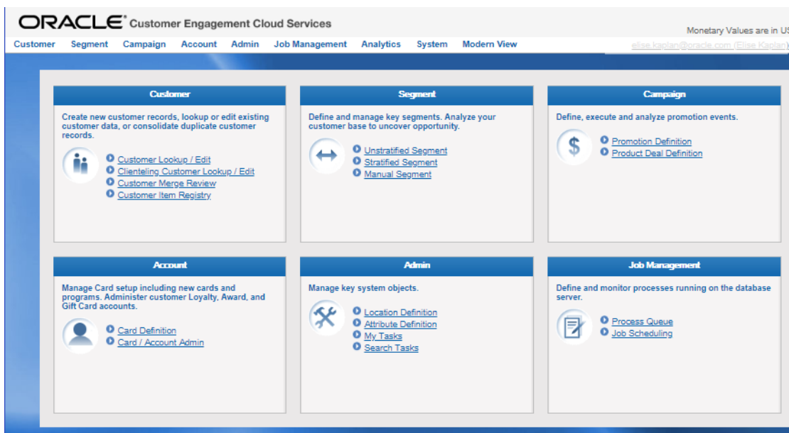
Figure 1-4: Main Page
