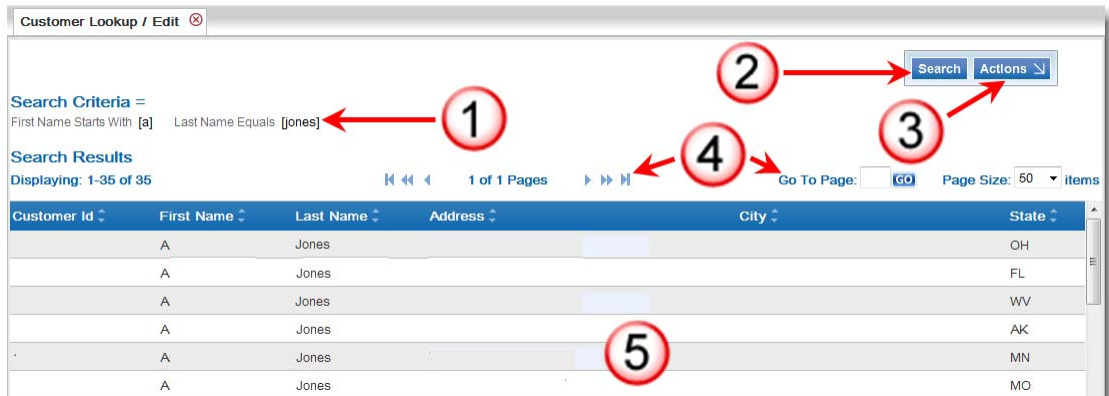
Figure 2-3: Customer List
