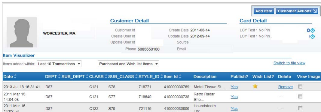
Figure 2-81: List View
