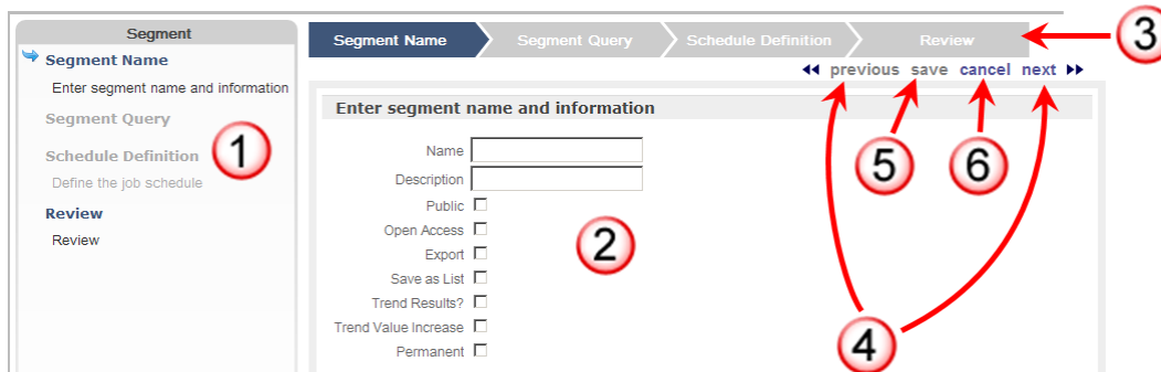
Figure 1-33: Sample Wizard
