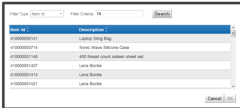
Figure 2-84: Search Results
