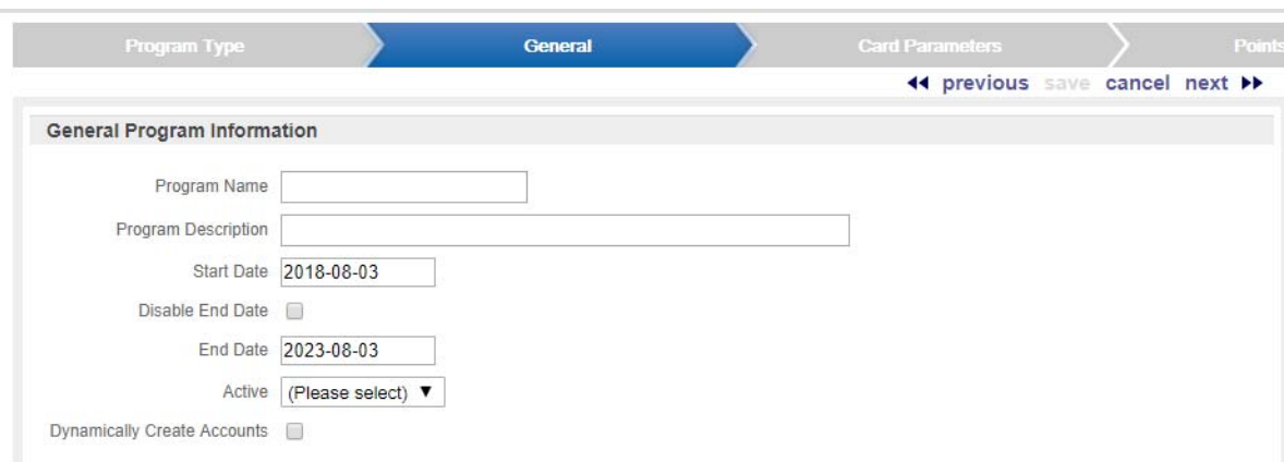
Figure 14-37: General Step
