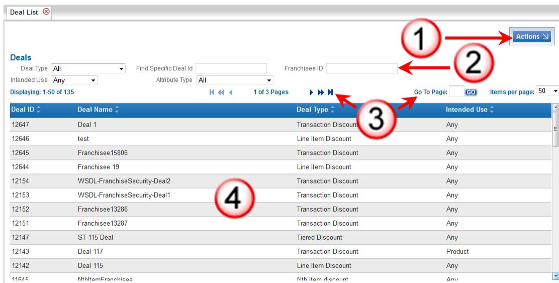
Figure 12-1: Deal List
