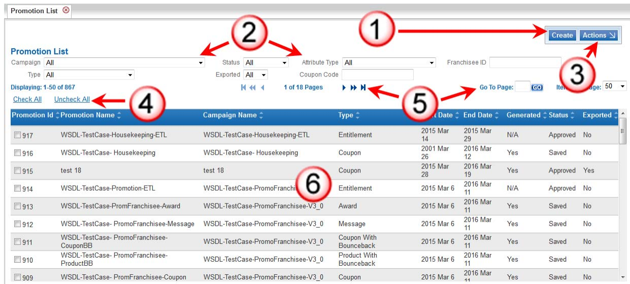
Figure 7-1: Promotions List
