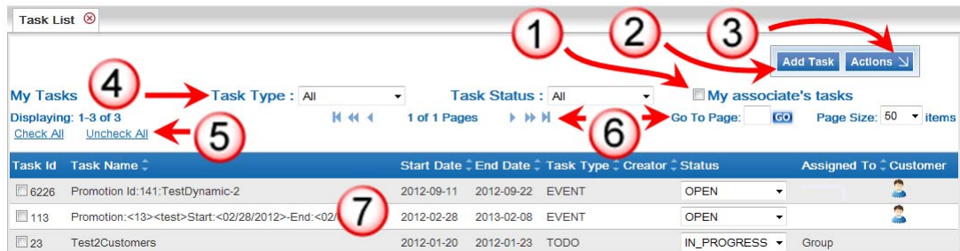
Figure 18-1: My Tasks
