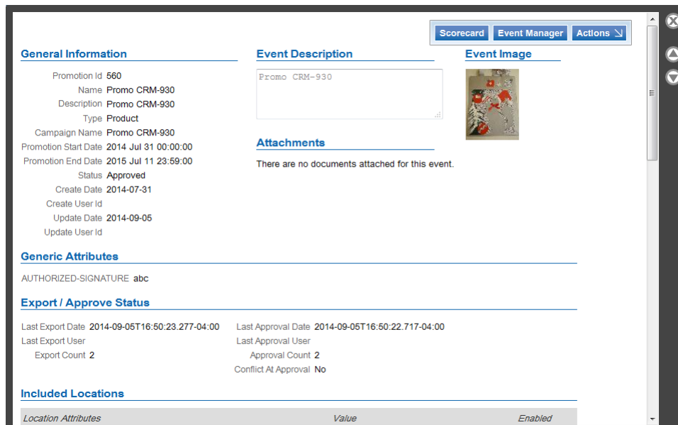
Figure 7-4: Promotion Window
