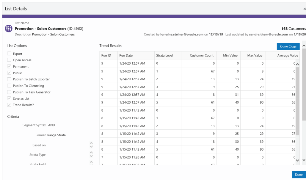
Figure 5–114 List Details Trend Results - Table
