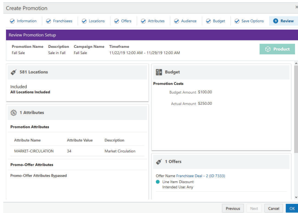
Figure 5–54 Review Tab
