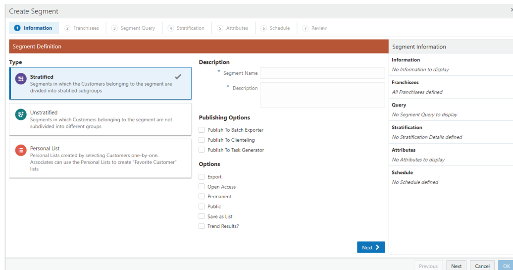
Figure 7–8 Information Tab
