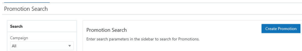
Figure 5–51 Promotion Search
