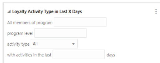
Figure 7–35 Segment
