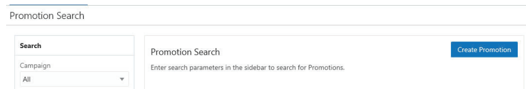
Figure 5–59 Promotion Search
