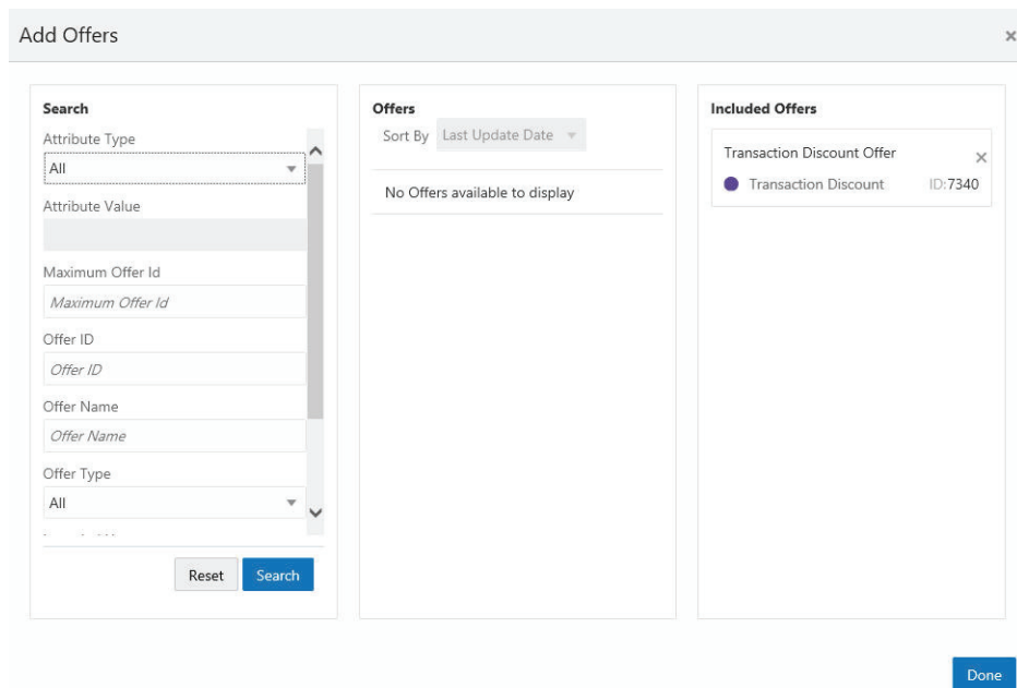
Figure 5–19 Add Offers
