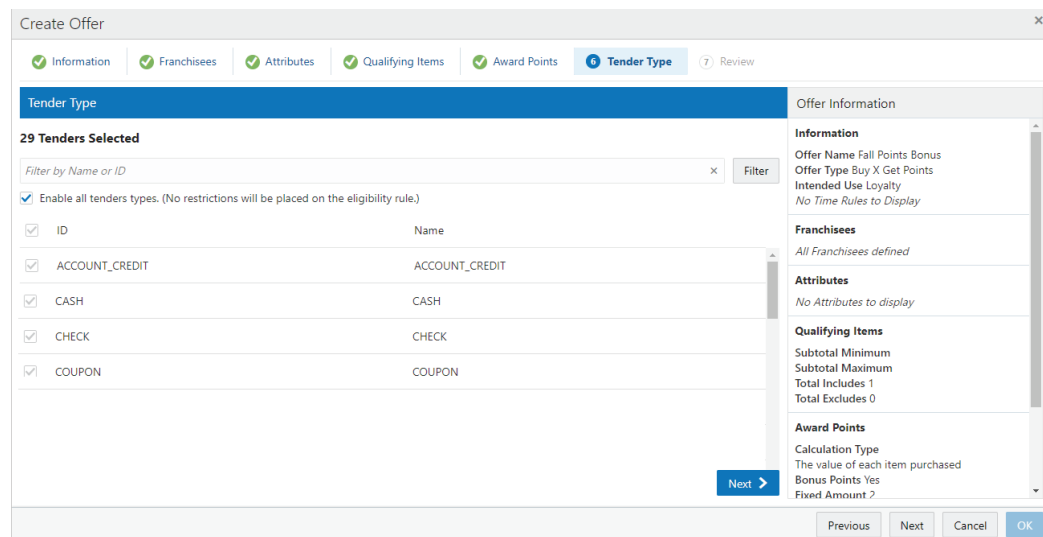
Figure 6–44 Tender Type
