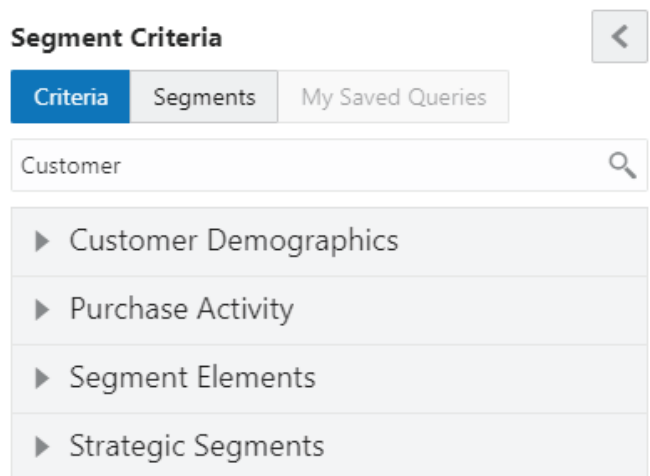
Figure 7–15 Criteria - Filtered
