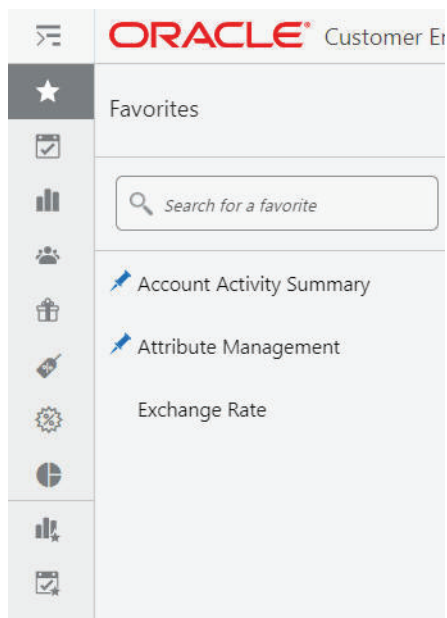
Figure 1–10 Favorites
