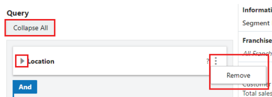
Figure 7–36 Query Options
