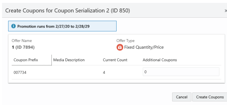
Figure 5–50 Create Coupons
