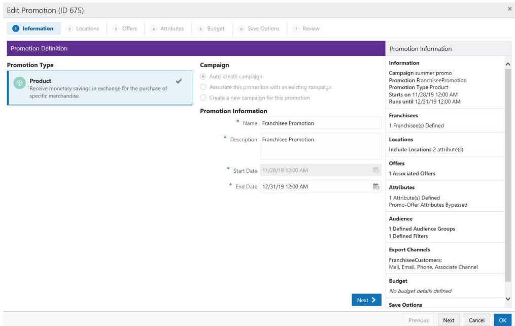
Figure 5–167 Edit Promotion
