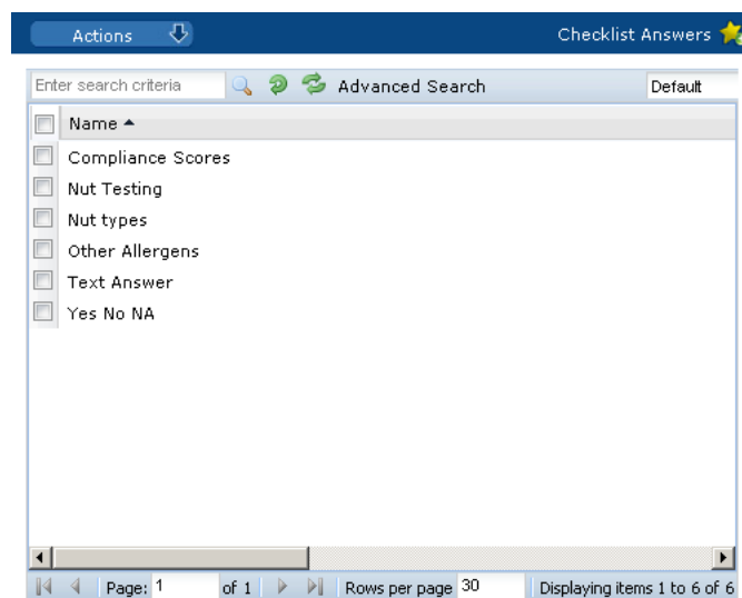
Figure 7–30 Checklist Answers
