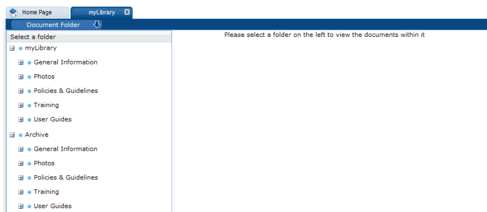
Figure 10–1 myLibrary Tab
