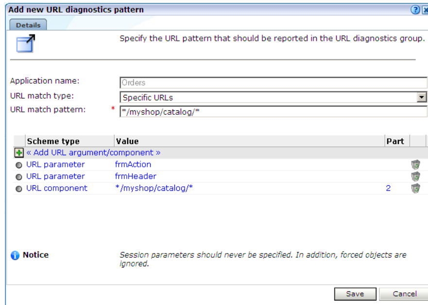
Figure 7–41 Edit URL Diagnostics Dialog
