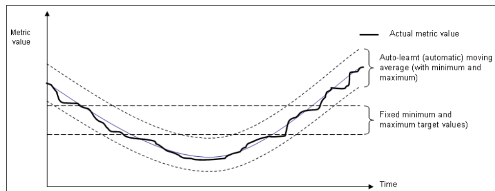
Figure 8-3 Automatic and Fixed KPI Targets Contrasted
