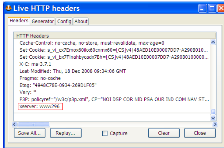
Figure Q-3 Example HTTP Header
