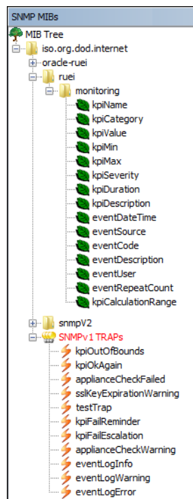
Figure 8–12 SNMP MIB Structure
