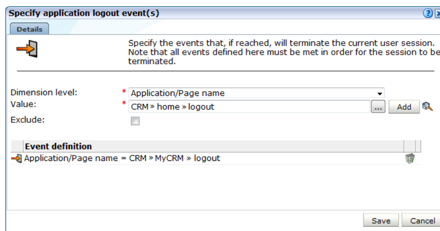
Figure 7-23 Specify Application Logout Event(s) Dialog
