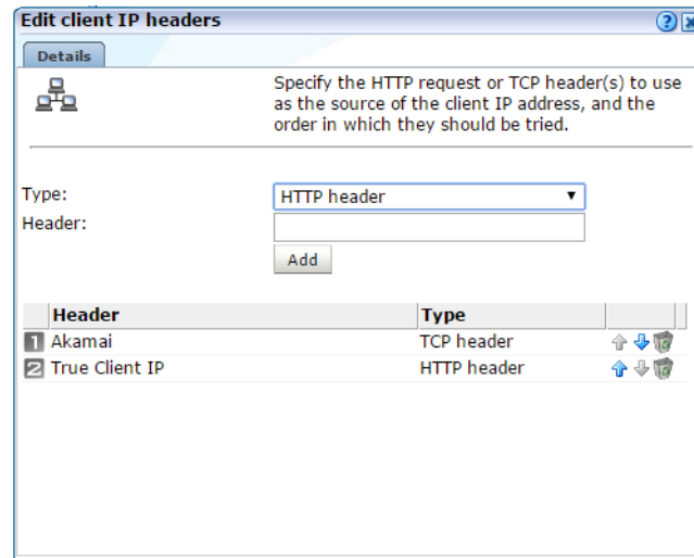
Figure Q-2 Edit Client IP Source
