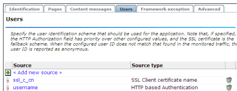
Figure 7-31 Application User Identification Scheme
