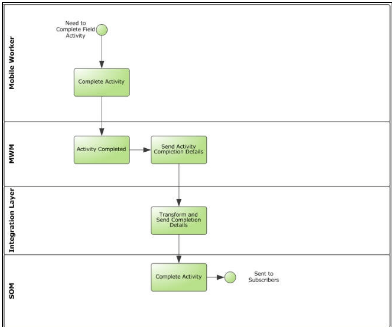
Activity Completion Business Process Diagram
