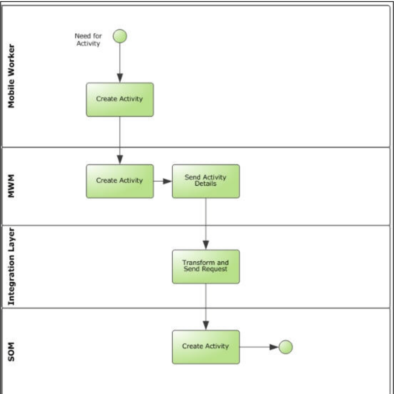
Create Activity Business Process Diagram
