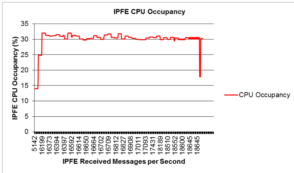
Figure 18 - IPFE CPU Occupancy
