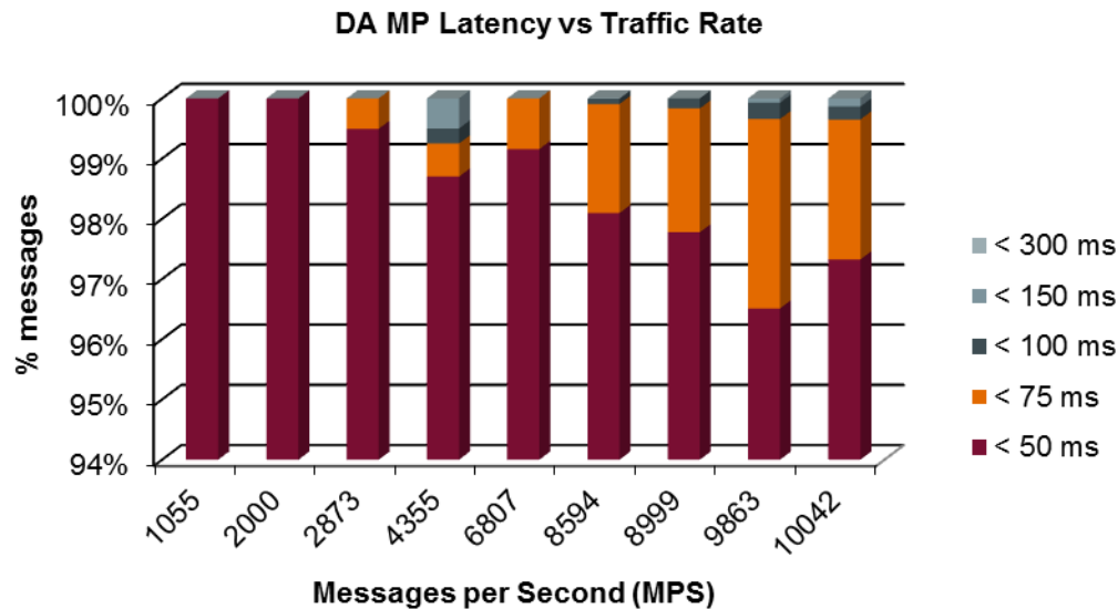
Figure 4 – DA-MP Round-Trip Latency
