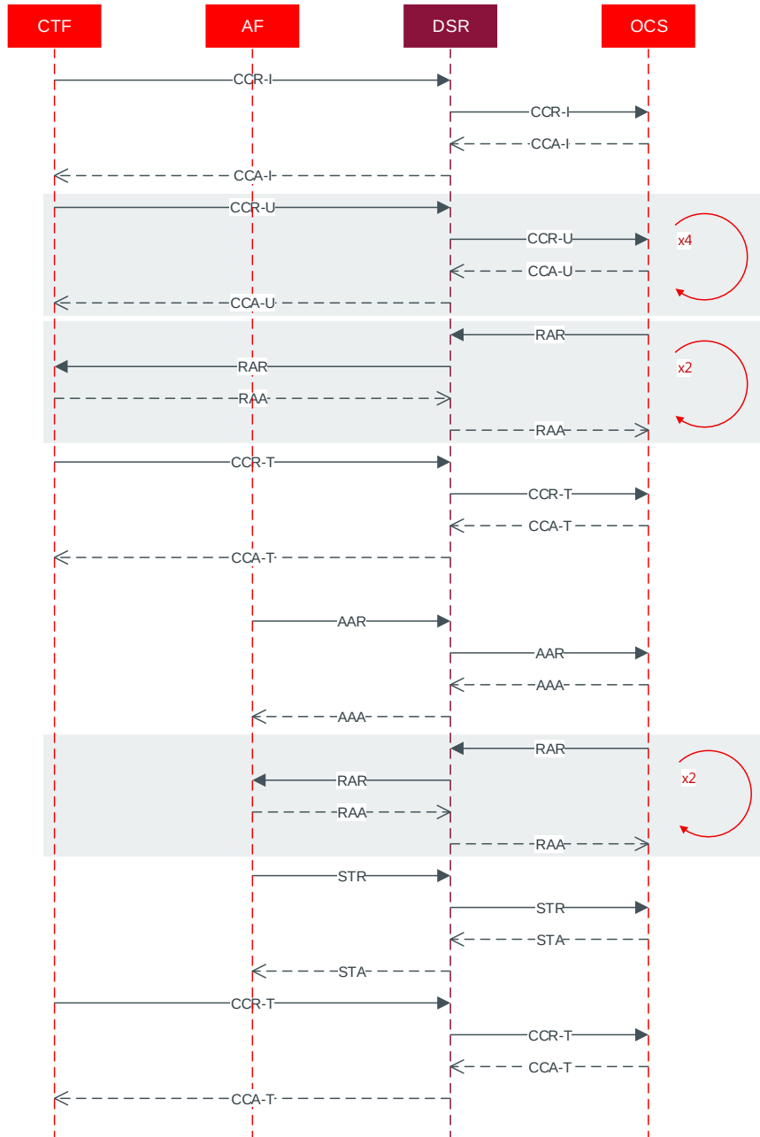
Figure 16 - SBR(b)Message Sequence
