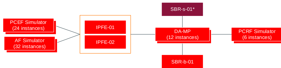
Figure 15 - SBR(b)Testing Topology
