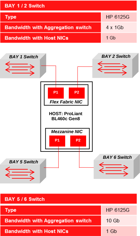
Figure 19 - Physical Networking for HP Gen8
