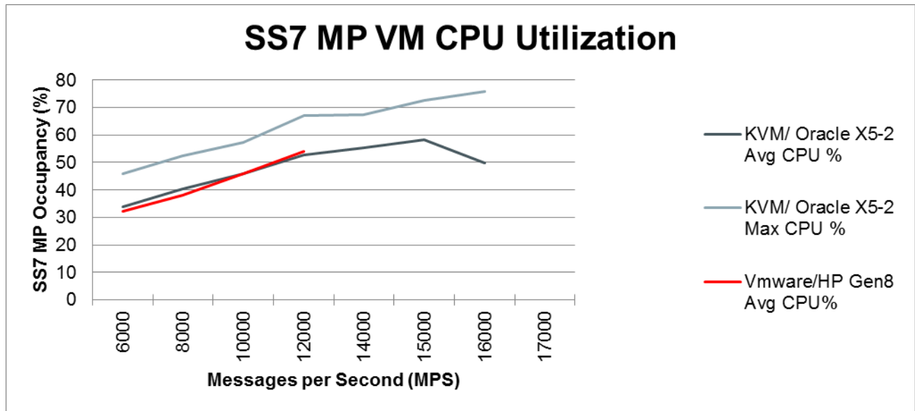
Figure 11 - SS7 MP CPU Occupancy(%) vs. MPS
