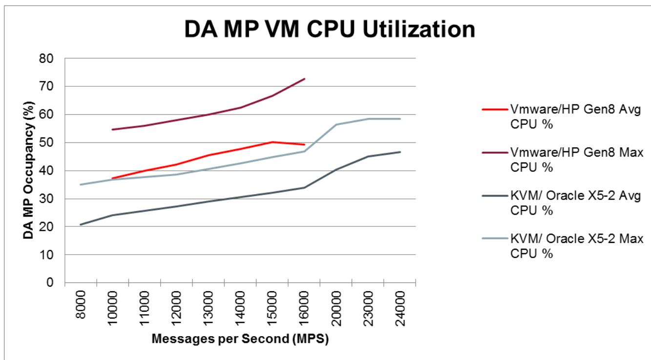
Figure 3 – DA-MP CPU Occupancy
