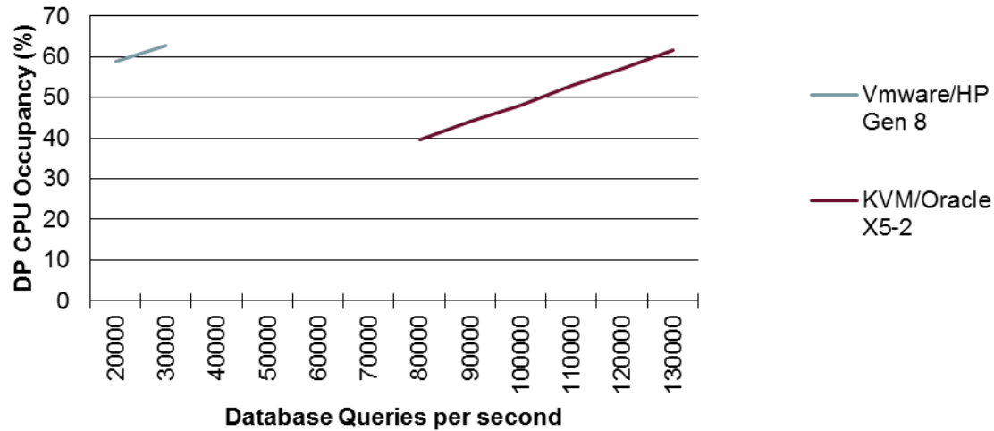
Figure 7 - DP CPU Util vs Traffic Rate (DP Queries)
