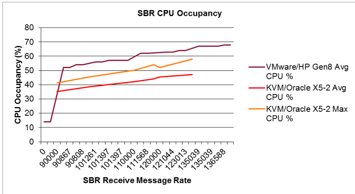
Figure 14 - SBR CPU Occupancy vs. Messages per Second
