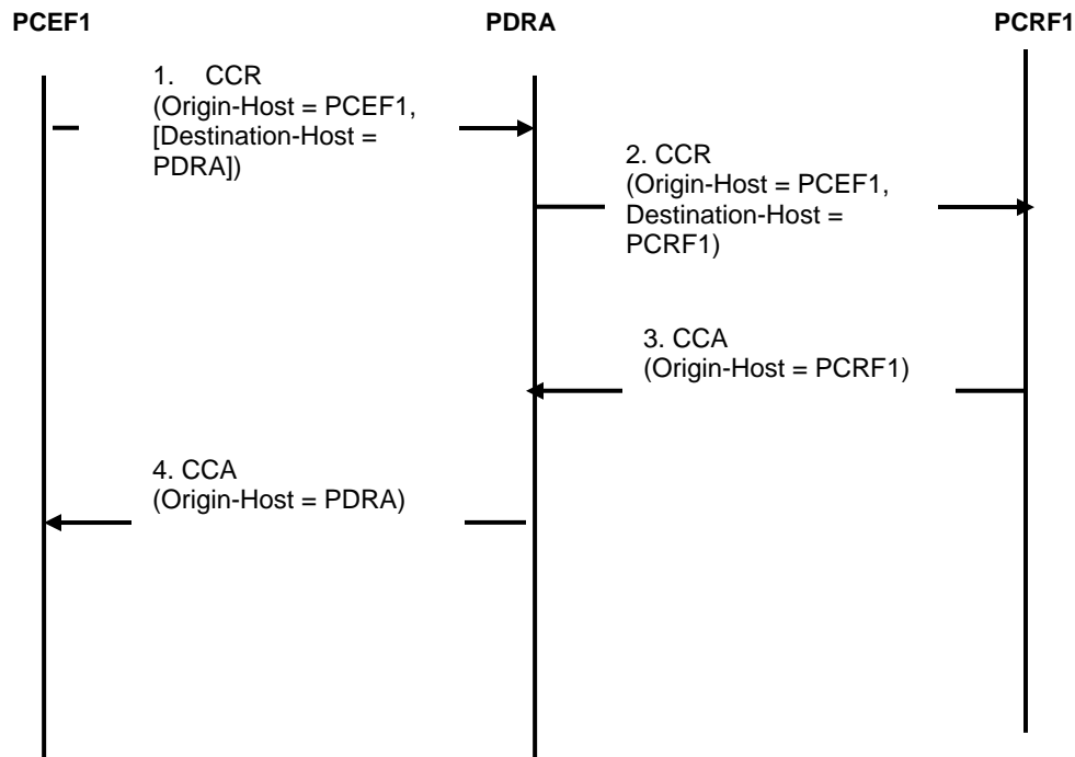
Figure 32 - PCRF topology hiding
