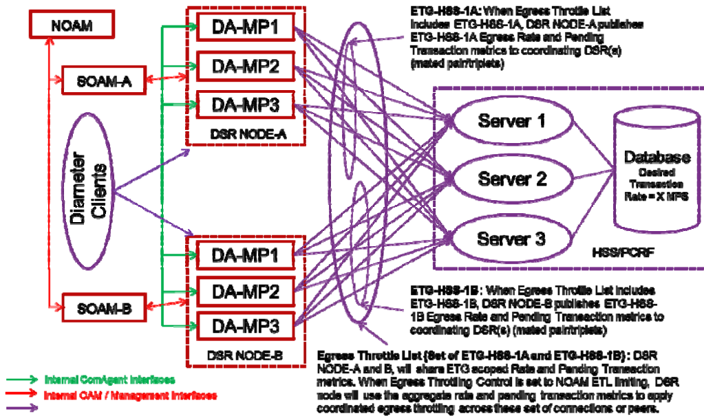
Figure 18 - 2 DSR Sites: Coordinated Egress Throttling Example
