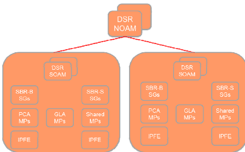
Figure 37 - PCA and GLA NOAM Architecture
