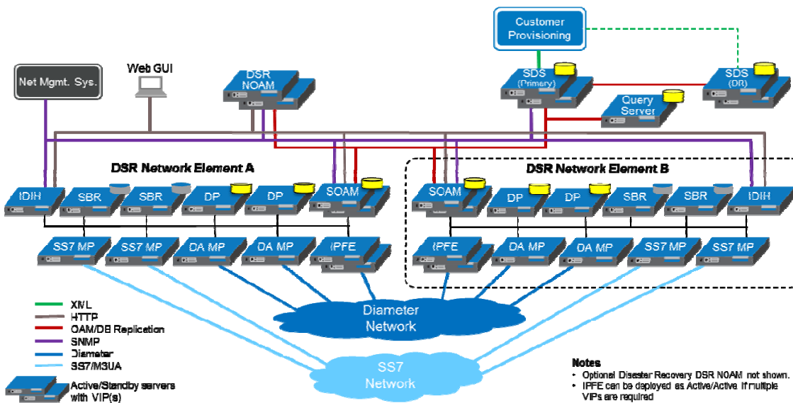
Figure 5 - DSR 7.x Architecture
