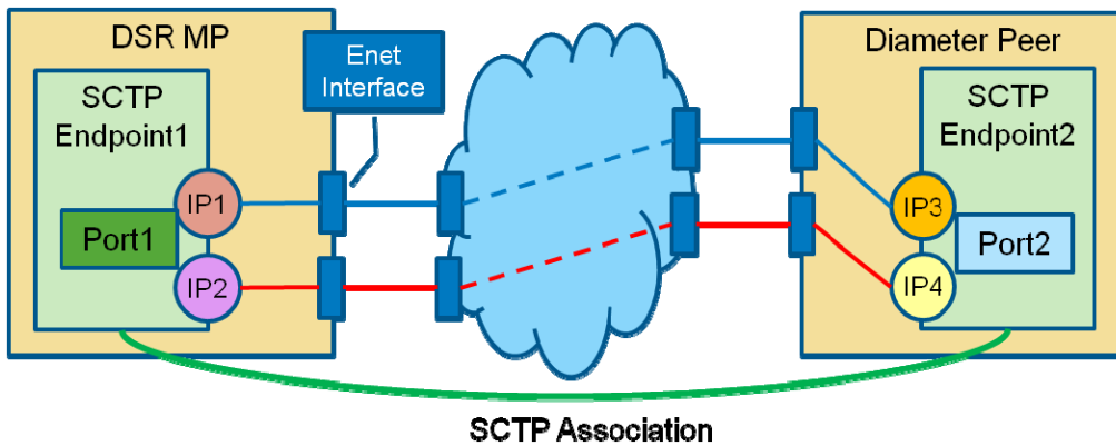
Figure 11 Sctp Multi-Homing
