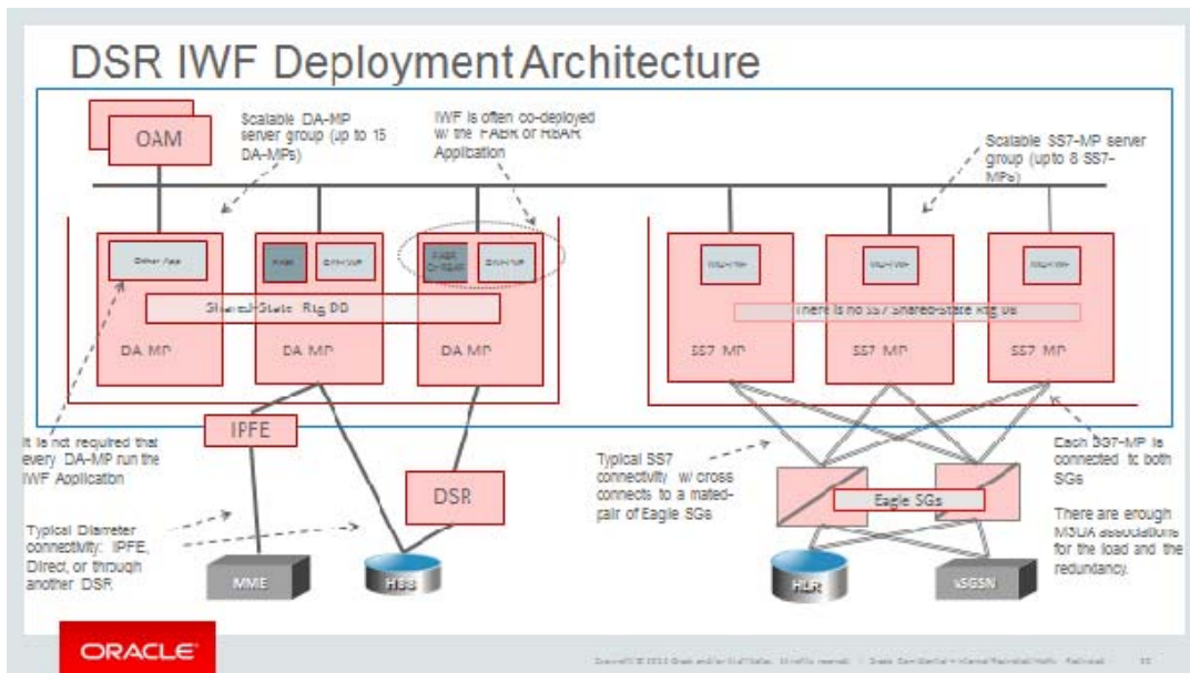
Figure 27 - DSR with MAP-Diameter IWF
