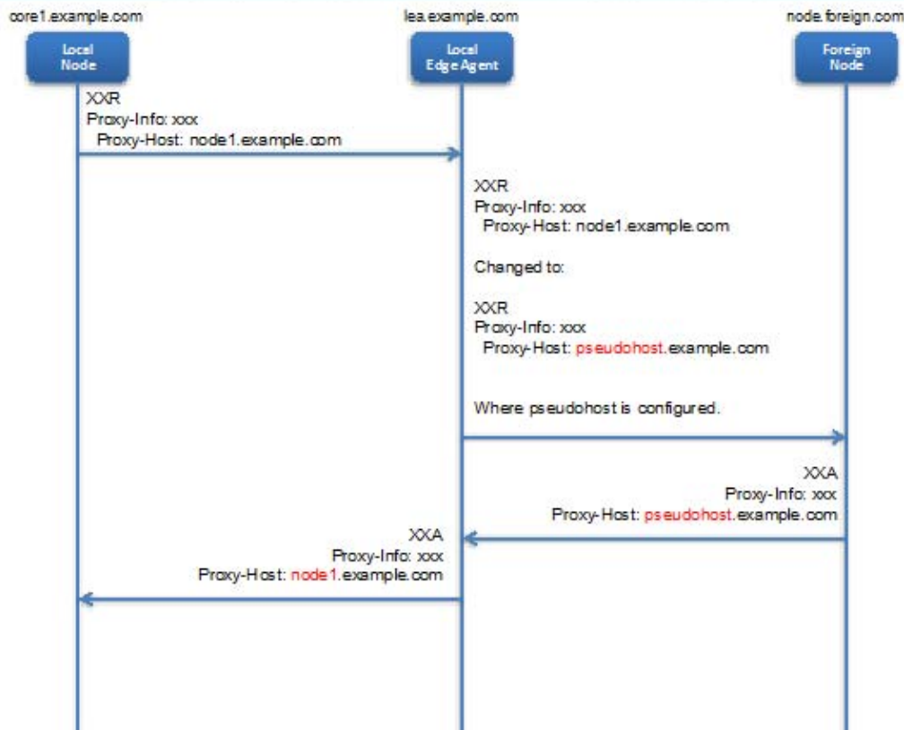
Figure 22 - Proxy-Host Topology Hiding Message Flow
