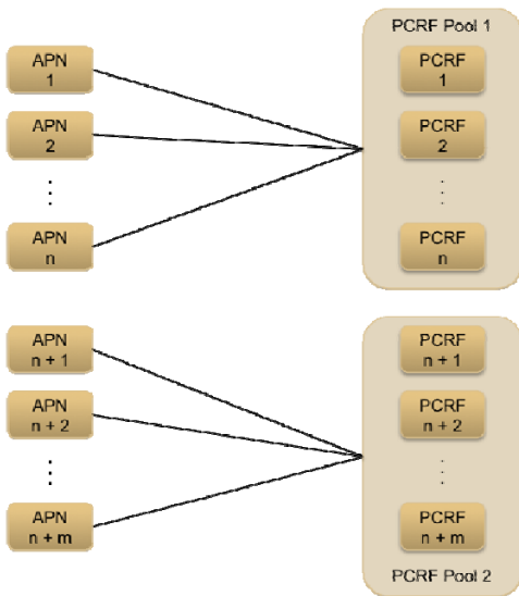
Figure 33 - Relationship between APNs and PCRF Pools
