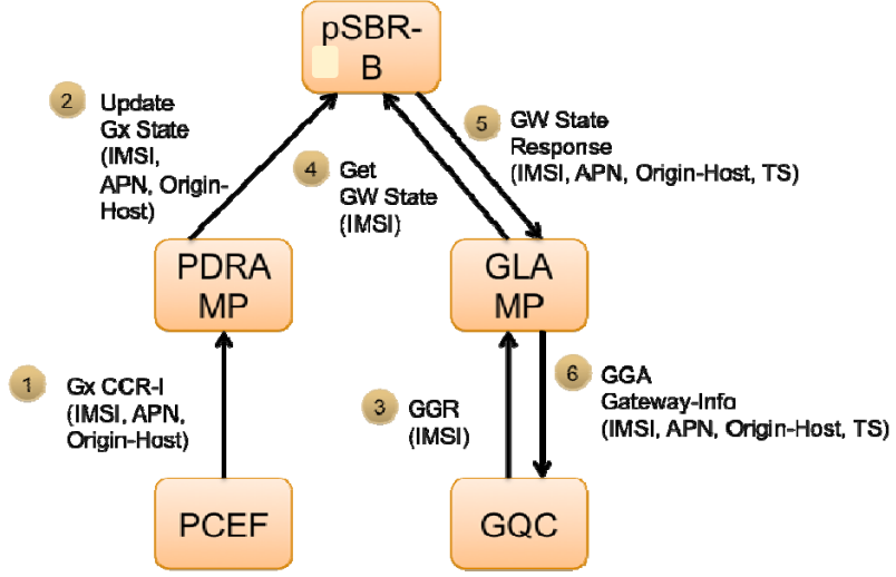
Figure 36 - IMSI Query with Single Matching Gx Session Use Case
