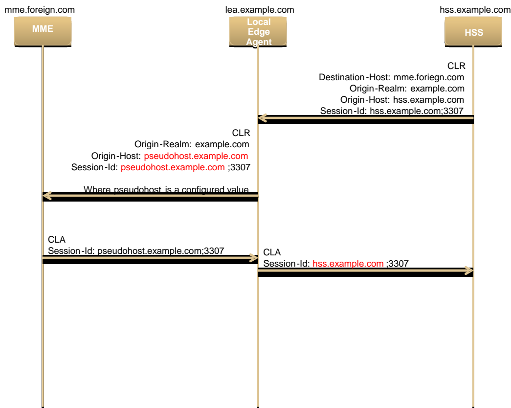
Figure 25 - S6a/S6d HSS Topology Hiding CLR Message Flow
