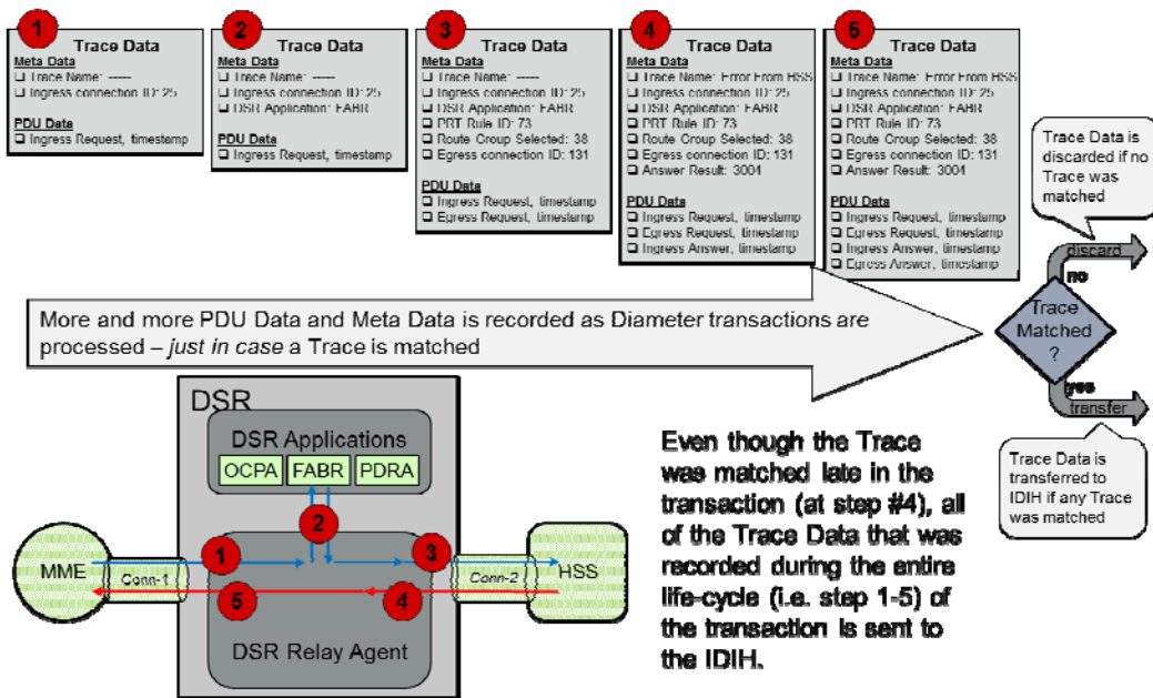
Figure 39 - IDIH Trace Data
