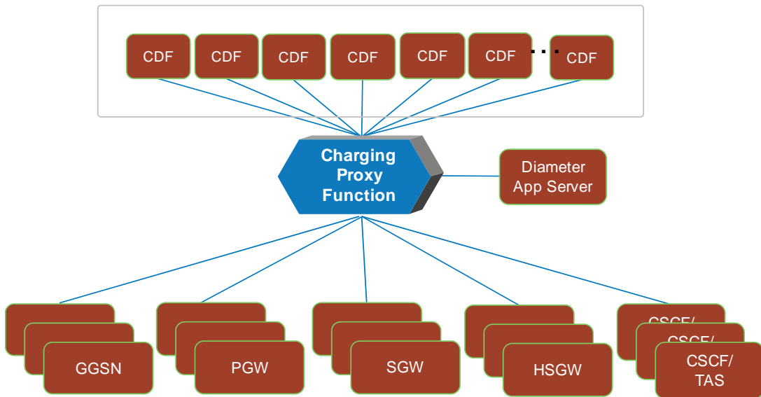
Figure 26 - Charging Proxy Network Architecture
