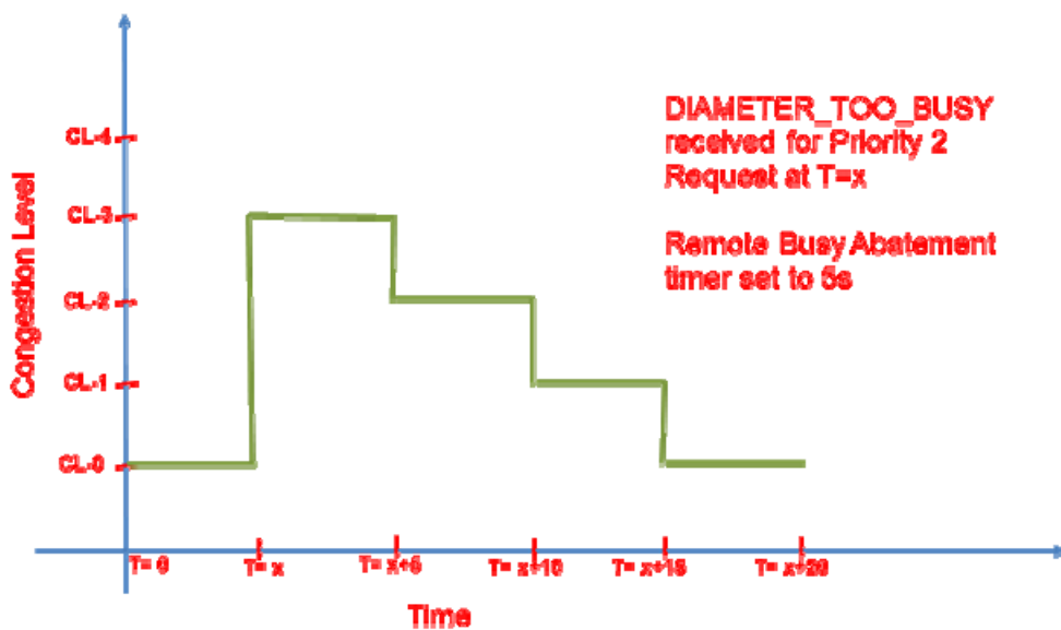
Figure 20 - Congestion level abatement over time for Remote Busy
