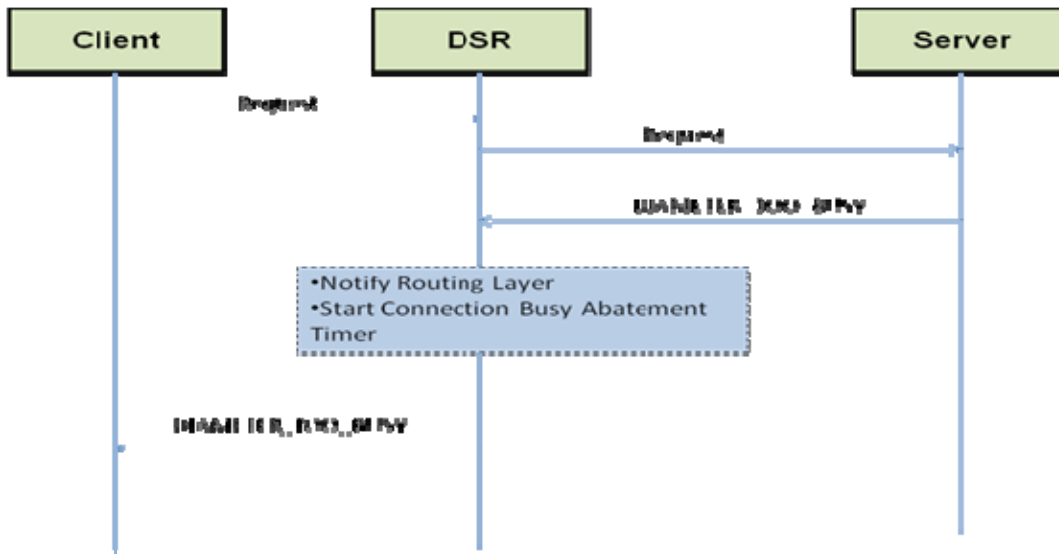
Figure 19 - Connection Busy
