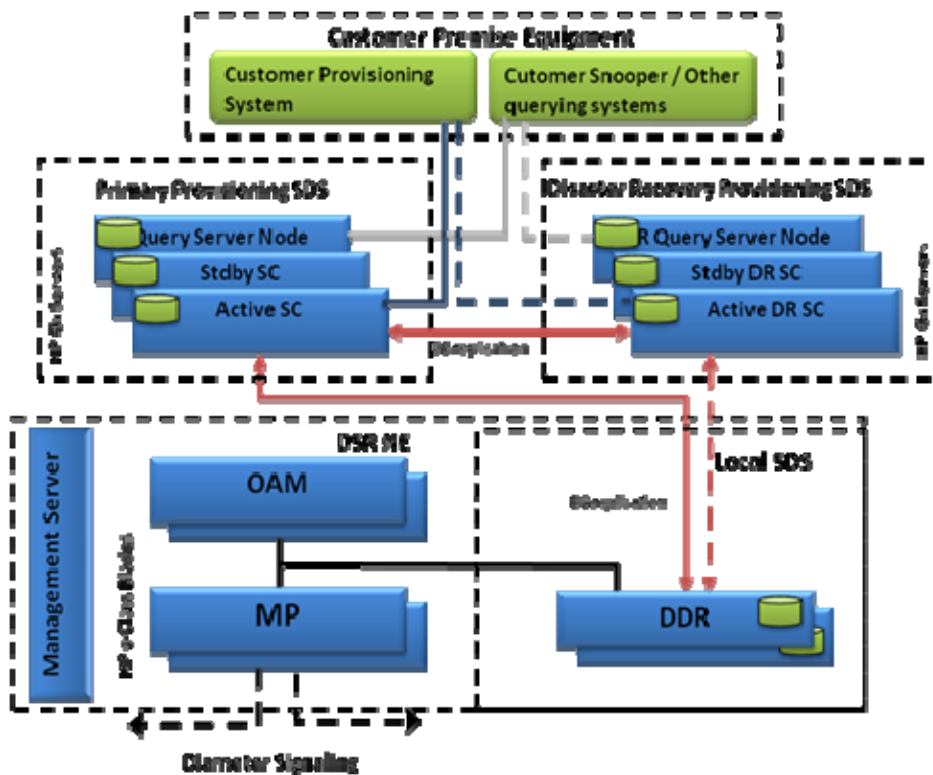
Figure 41 - Subscriber Data Server Architecture
