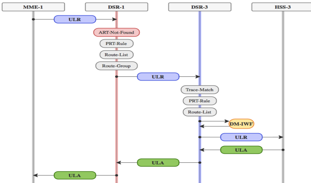
Figure 40 - Message Flow for Network Wide Trace
