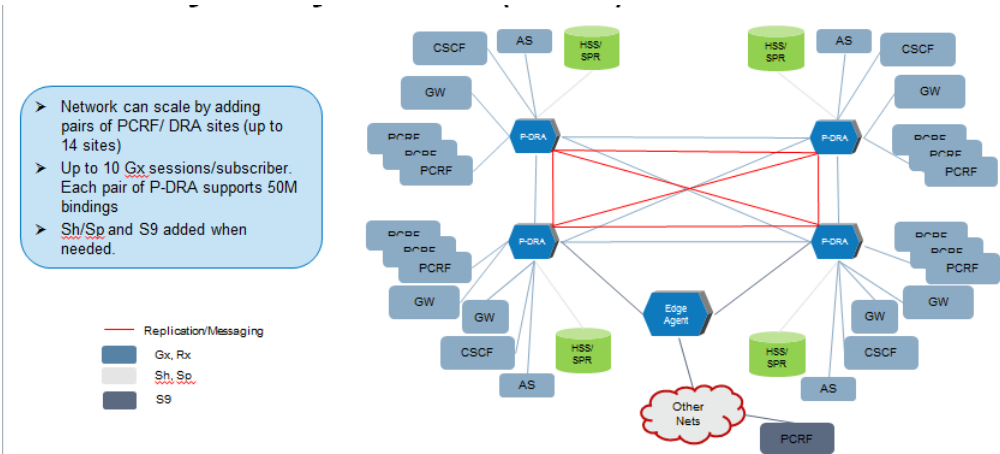
Figure 35 - PCA Example Deployment
