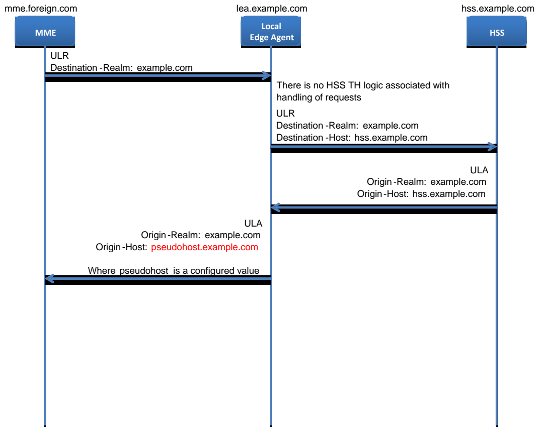
Figure 24 - S6a/S6d HSS Topology Hiding - ULR Message Flow
