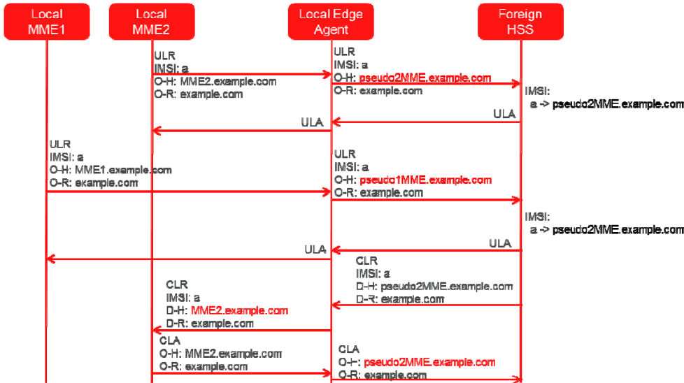
Figure 23 - MME/SGSN Topology Hiding
