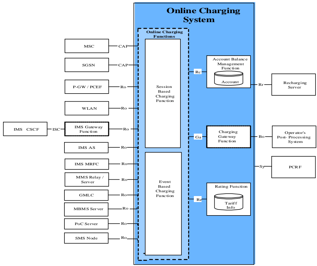
Figure 28 - Online Charging System and Architecture
