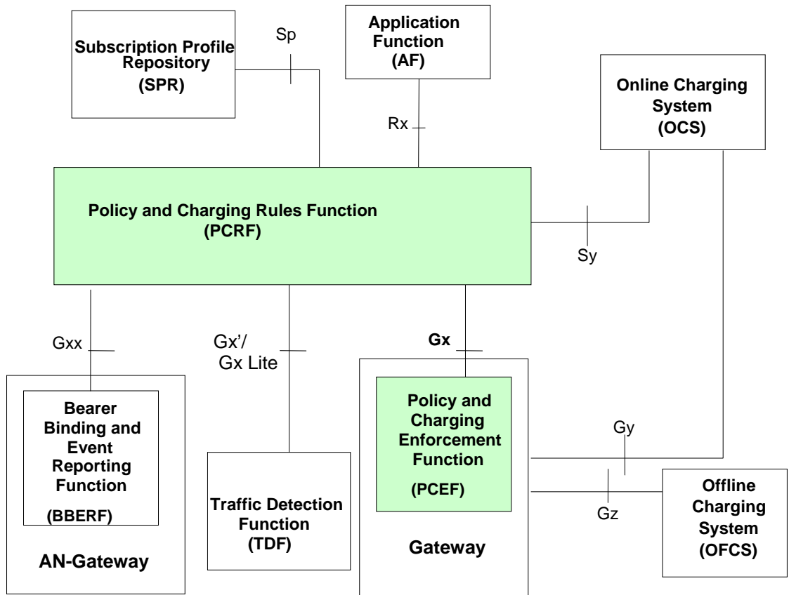
Figure 31 - Overall PCC logical architecture (non-roaming)
