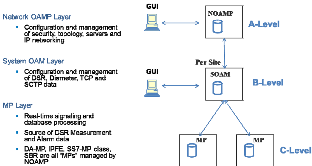
Figure 42 - DSR 3-tiered Topology Architecture
