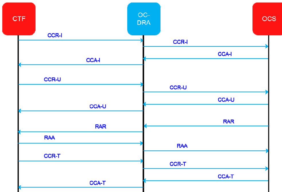
Figure 29: A typical Online Charging Session
