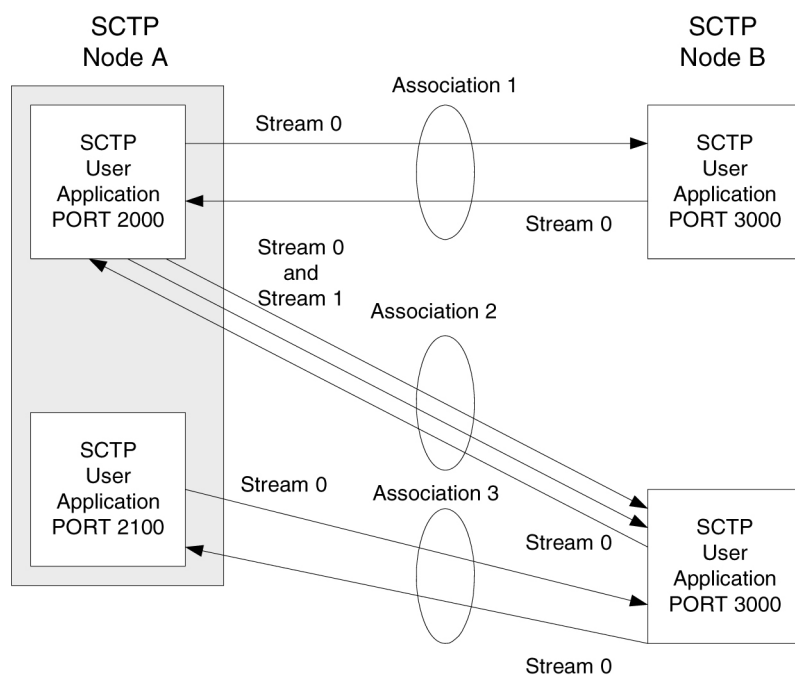
Figure 18: SCTP Connectivity
