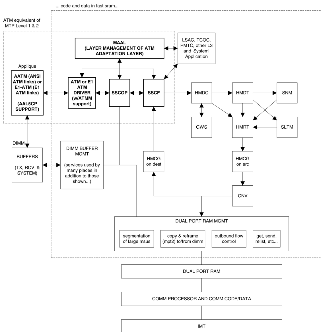
Figure 36: Functional Block Diagram of ATM High-Speed Signaling Link
