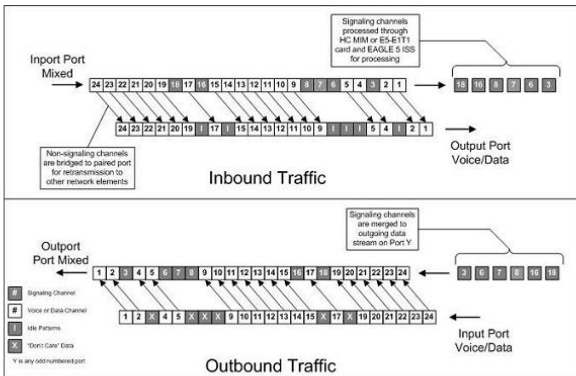
Figure 31: Channel Bridging
