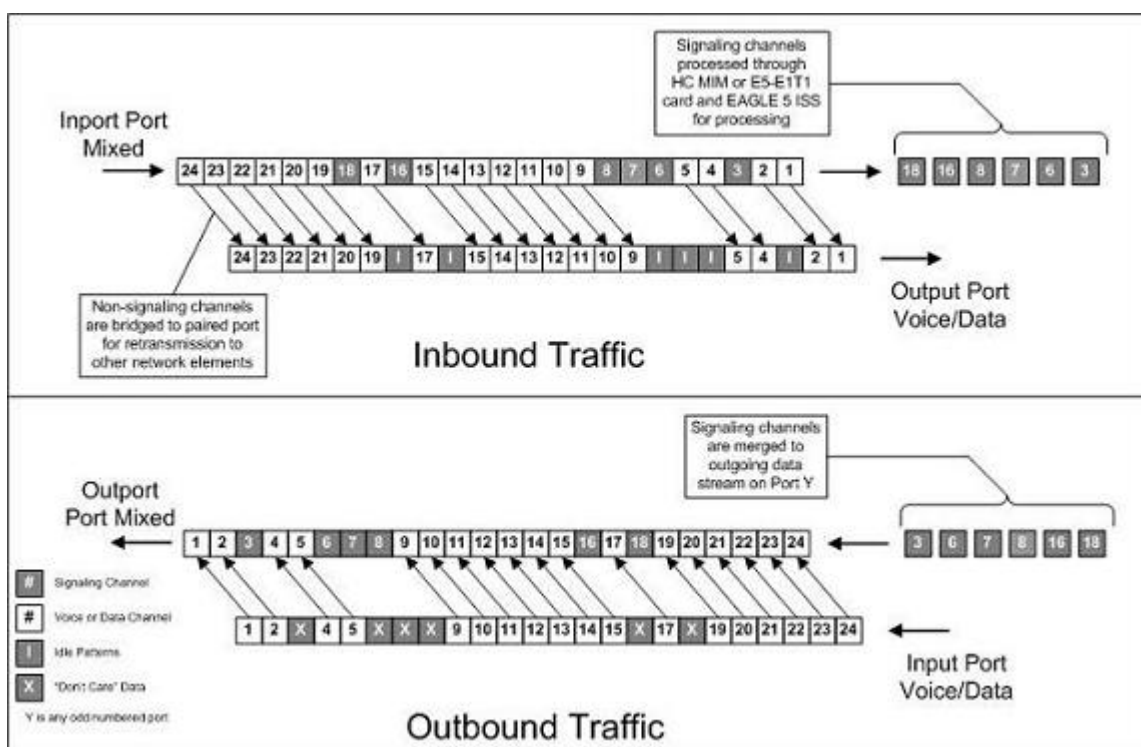
Figure 28: Channel Bridging
