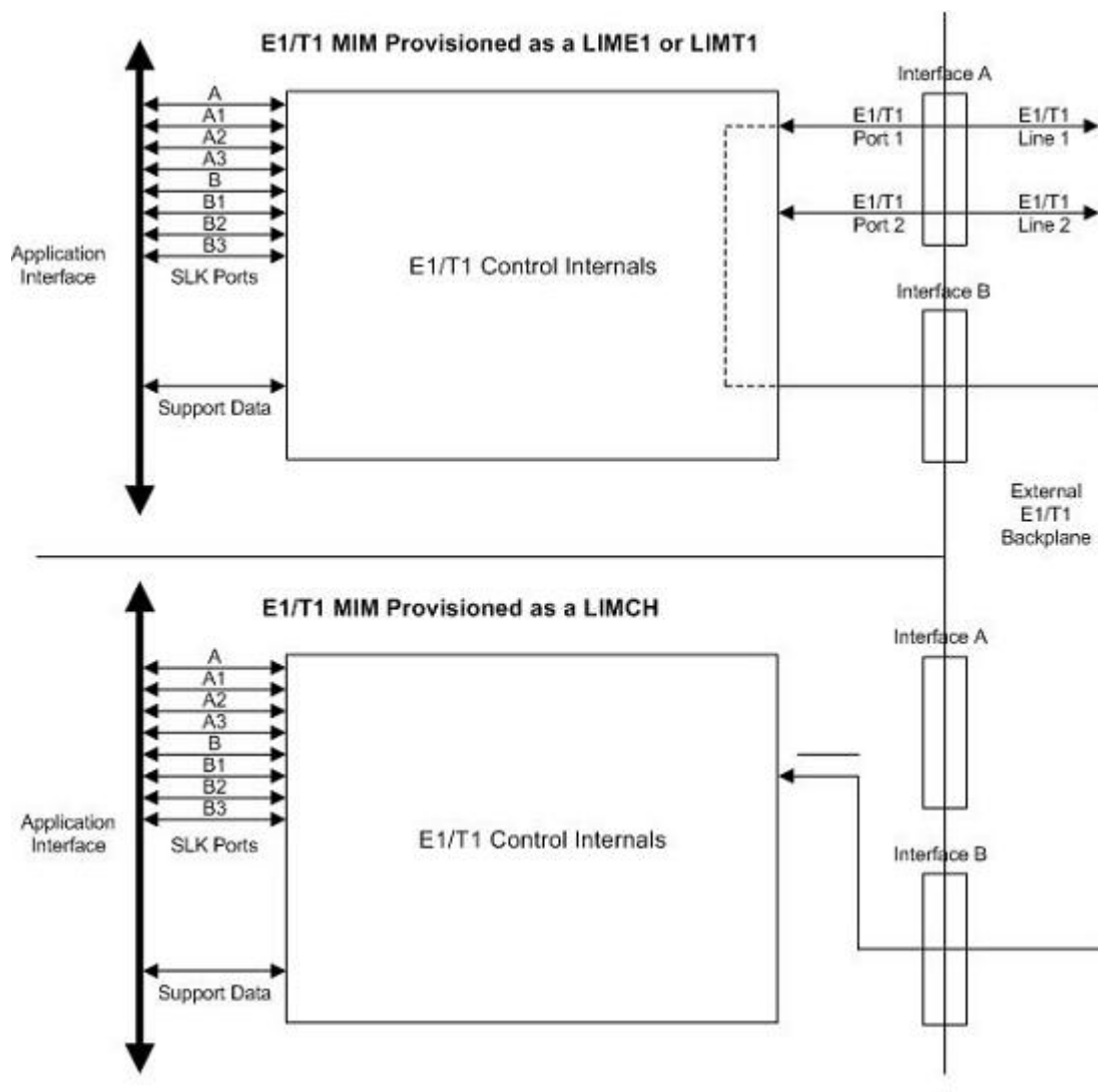
Figure 29: E1/T1 MIM Block Diagram
