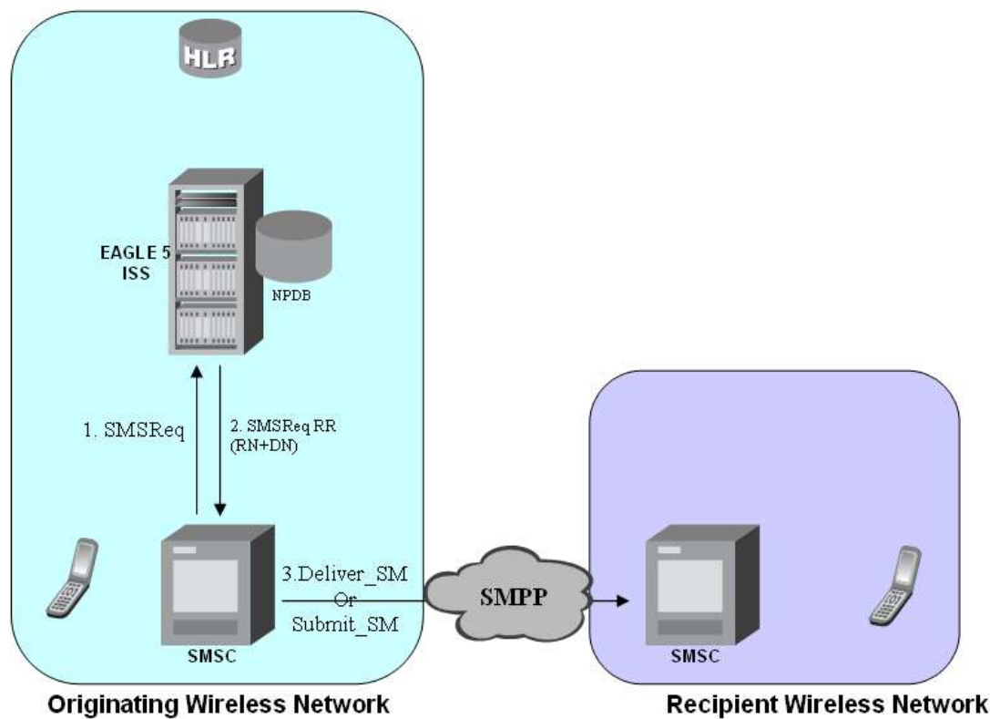
Figure 3: MT-Based IS41 SMS NP Call Flow for Other-Network Subscriber
