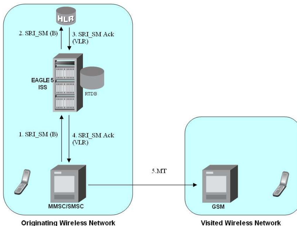
Figure 8: MT-Based GSM SMS and MMS NP Call Flow for In-Network Subscriber
