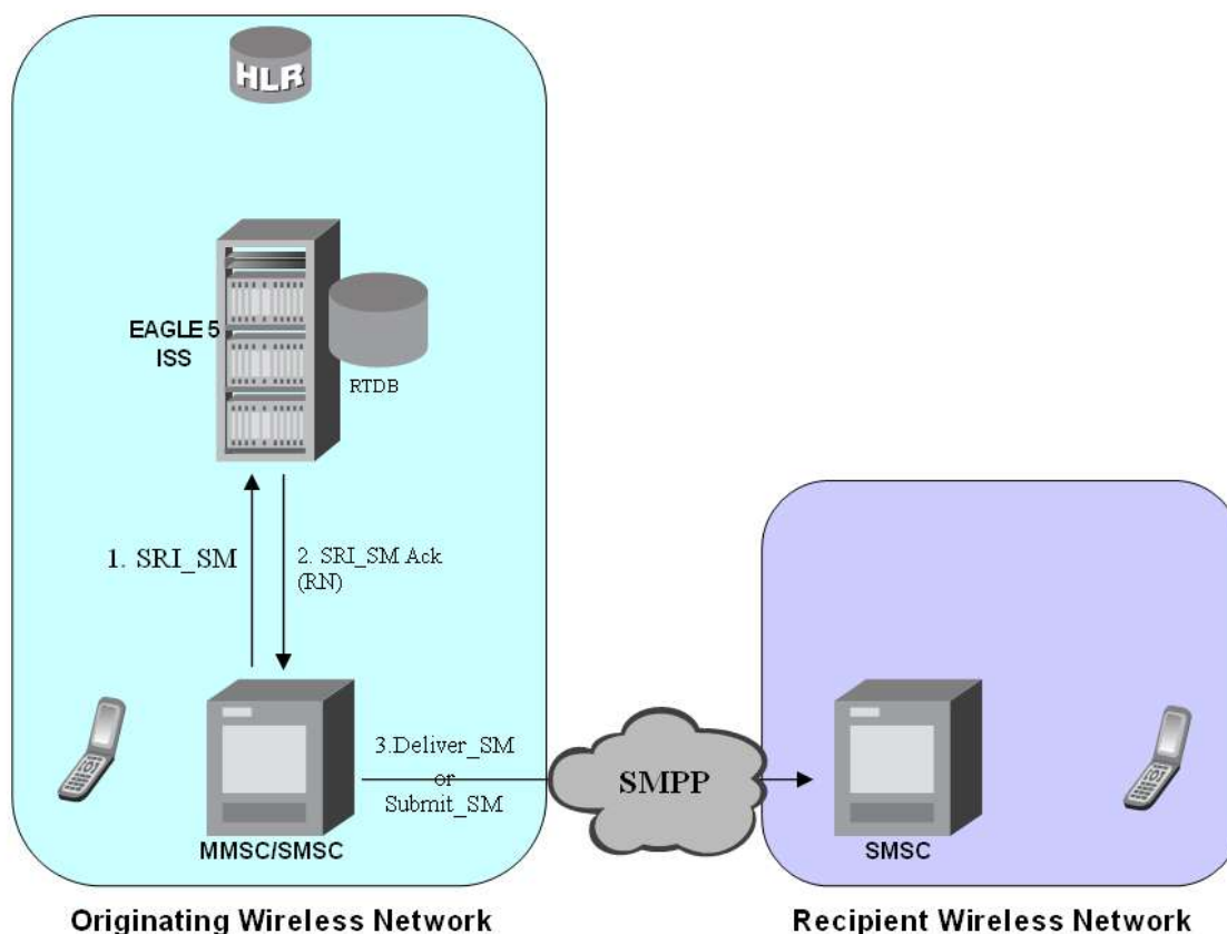
Figure 9: MT-Based GSM SMS and MMS NP Call Flow for Other-Network Subscriber
