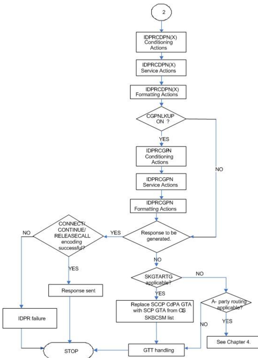
Figure 3: Message Flow for IDP Relay - Sheet 3 of 3
