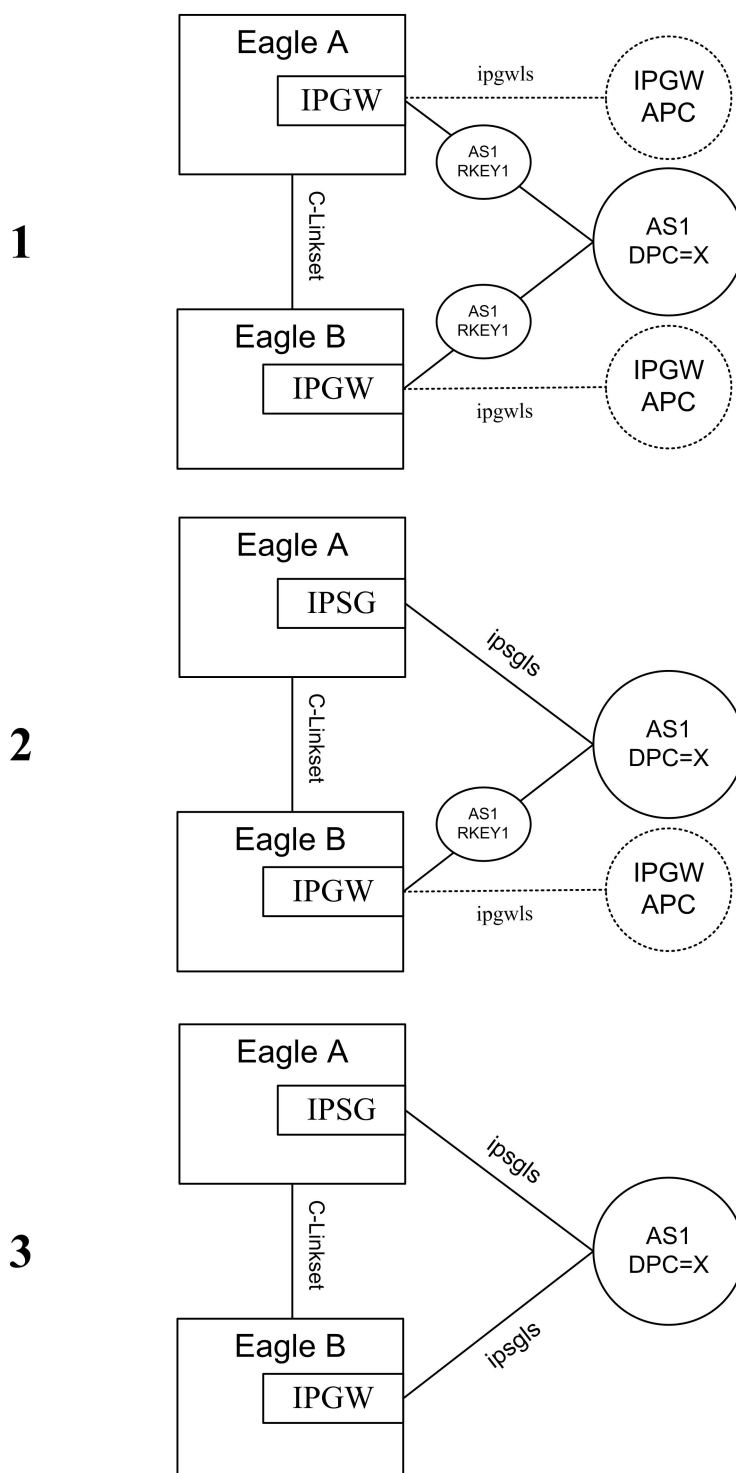
Figure 13: IPGWx to IPSPG-M3UA Conversion Strategy Example 1
