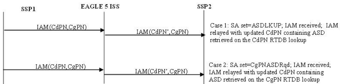
Figure 25: ISUP IAM Message Flows for TIF ASD for TIF CdPN Service
