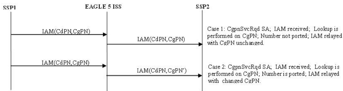
Figure 9: ISUP Message Flows for TIF NP CgPN Portability
