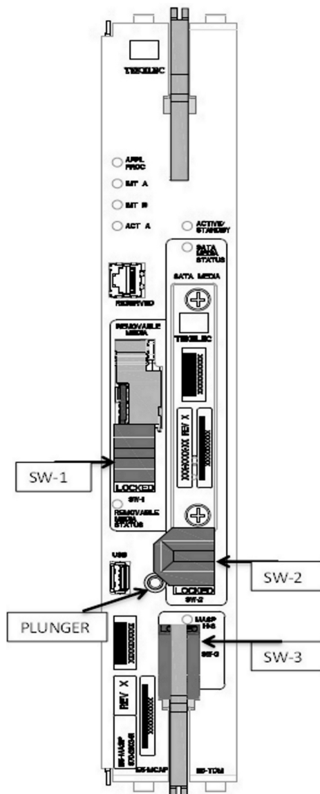
Figure 33: E5-MASP Card (870-2903-02)
