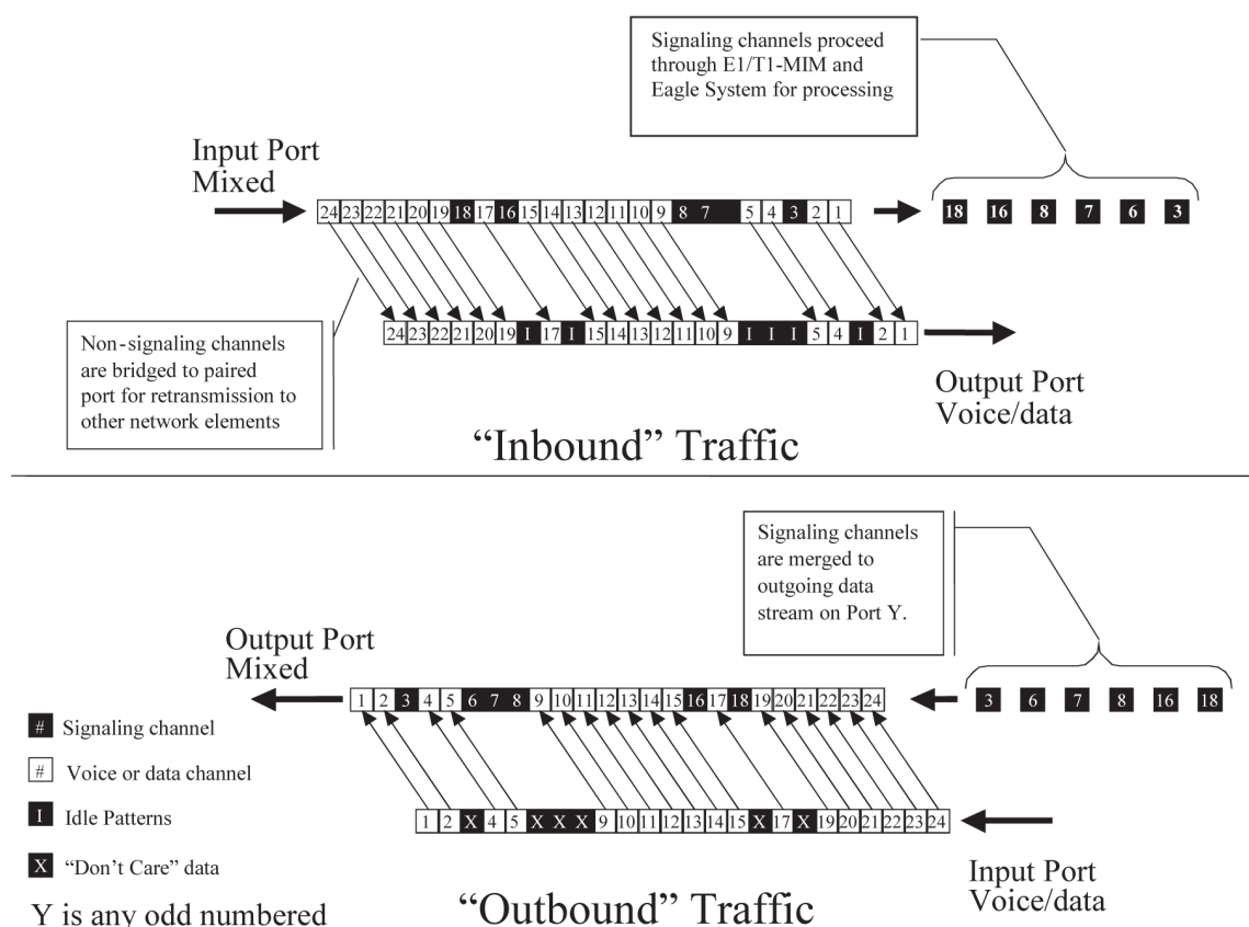
Figure 46: Channel Bridging Schematic
