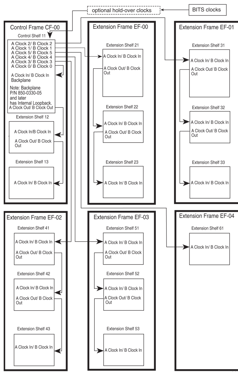
Figure 6: Clock Routing
