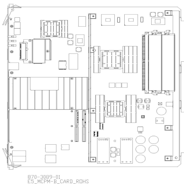
Figure 39: E5-MCPM-B
