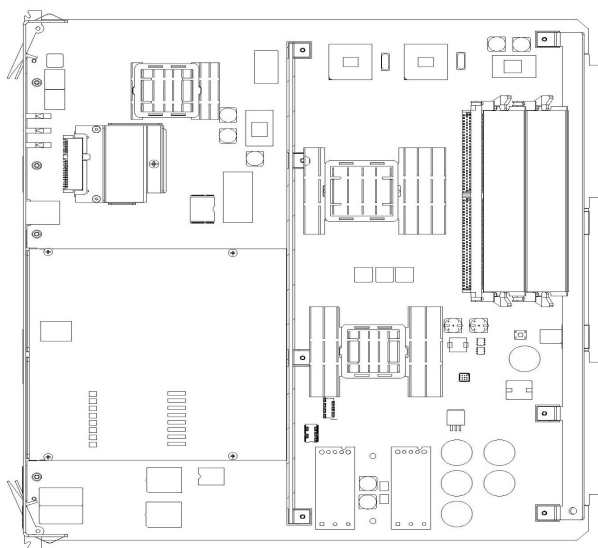
870-2972-01 E5_ATM-B_CARD_RDHS
