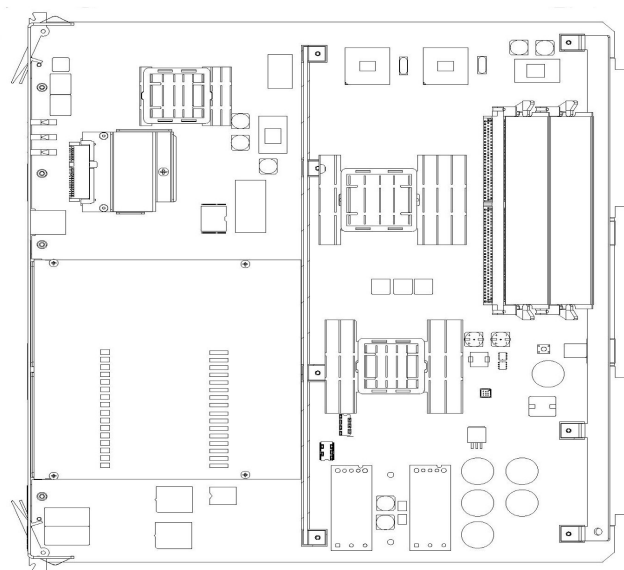
870-2970-01 E5_E1T1-B_CARD_RDHS
