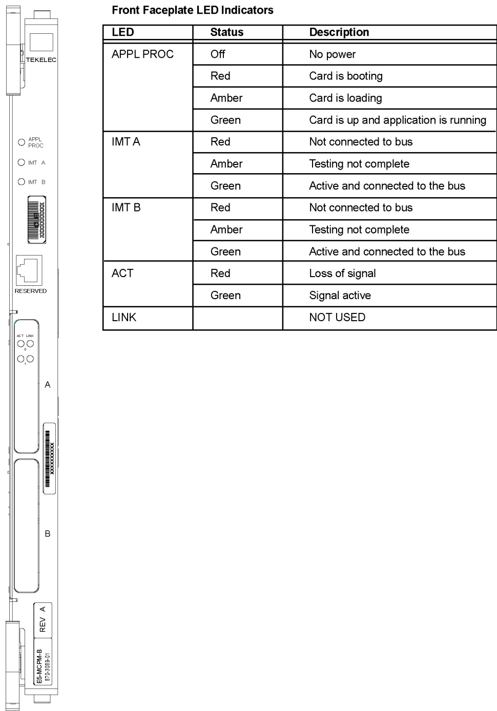
Figure 50: E5-MCPM-B
