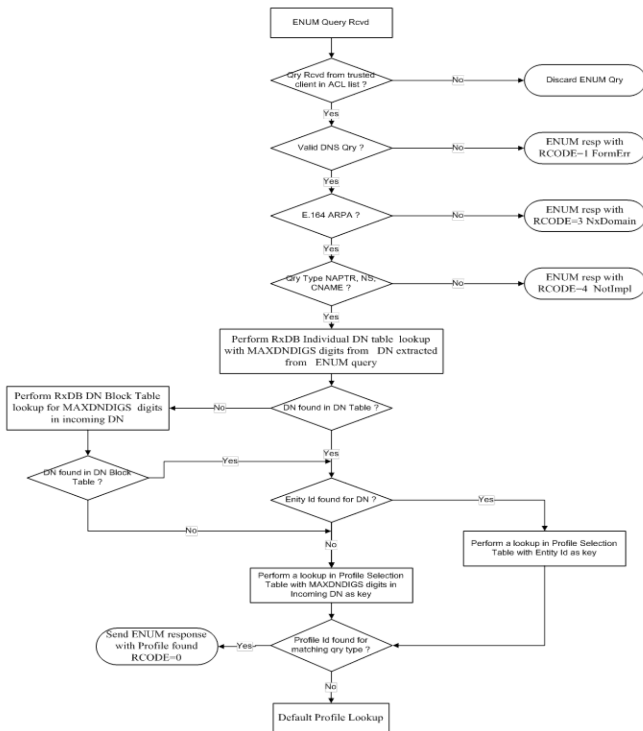
Figure 4: ENUM Message Flow for MNP
