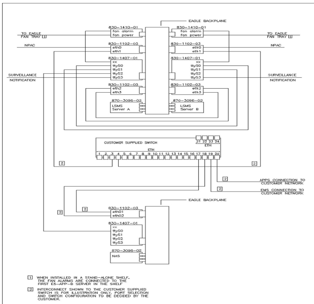
Figure 19: LSMS and NAS Segmented Connections
