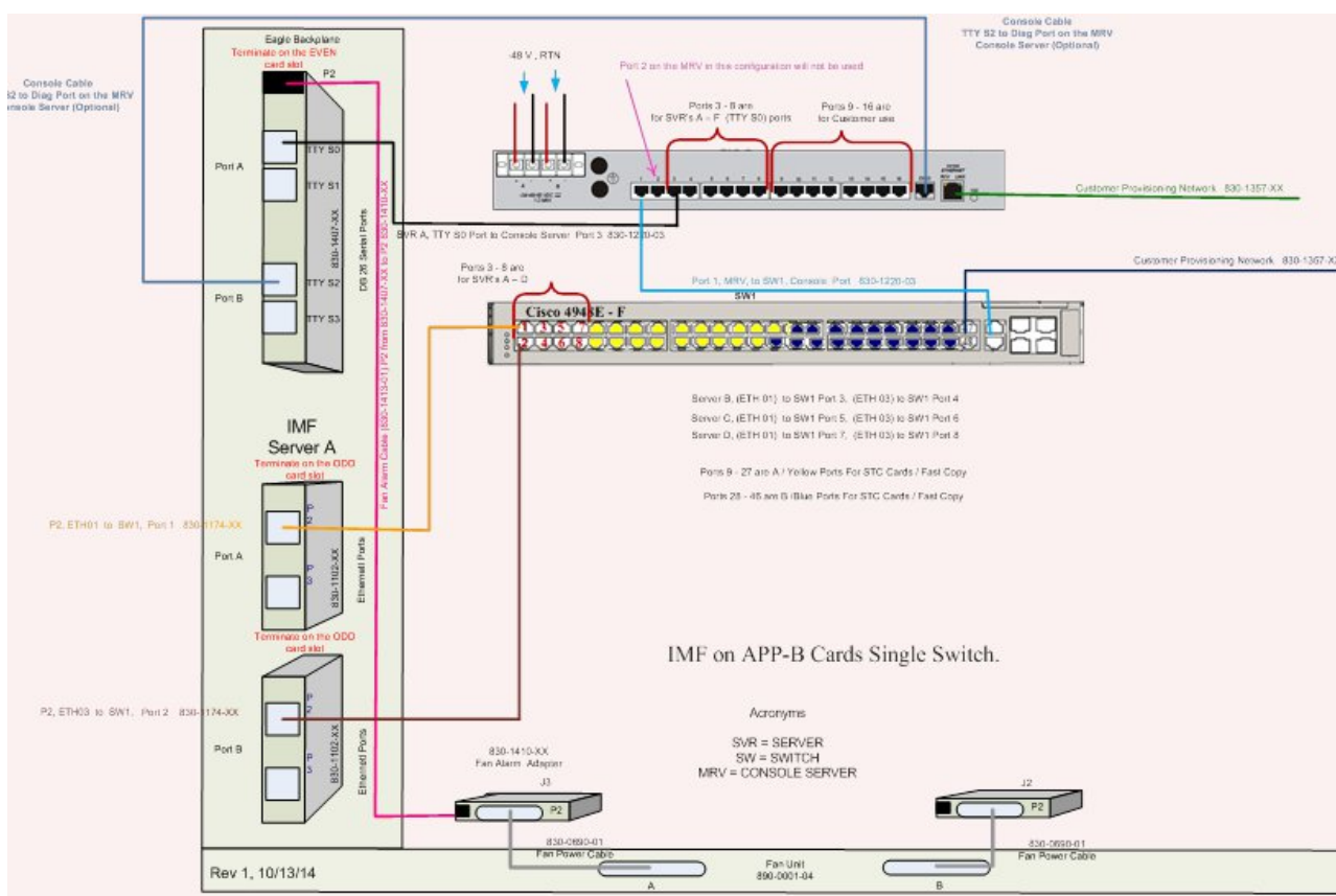
Figure 20: IMF Interconnect Single Switch Configuration
