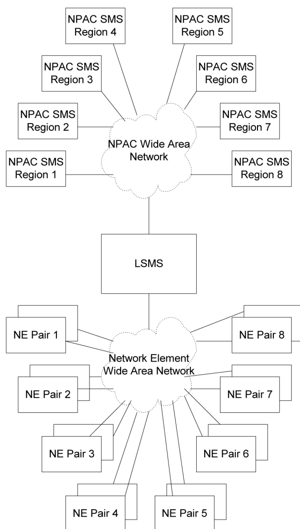
Figure 1: LNP Configuration
