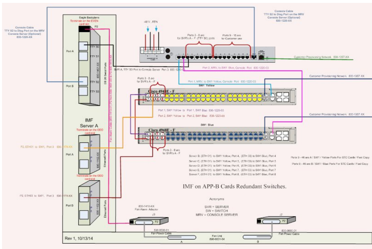
Figure 21: IMF Interconnect Dual Switch Configuration
