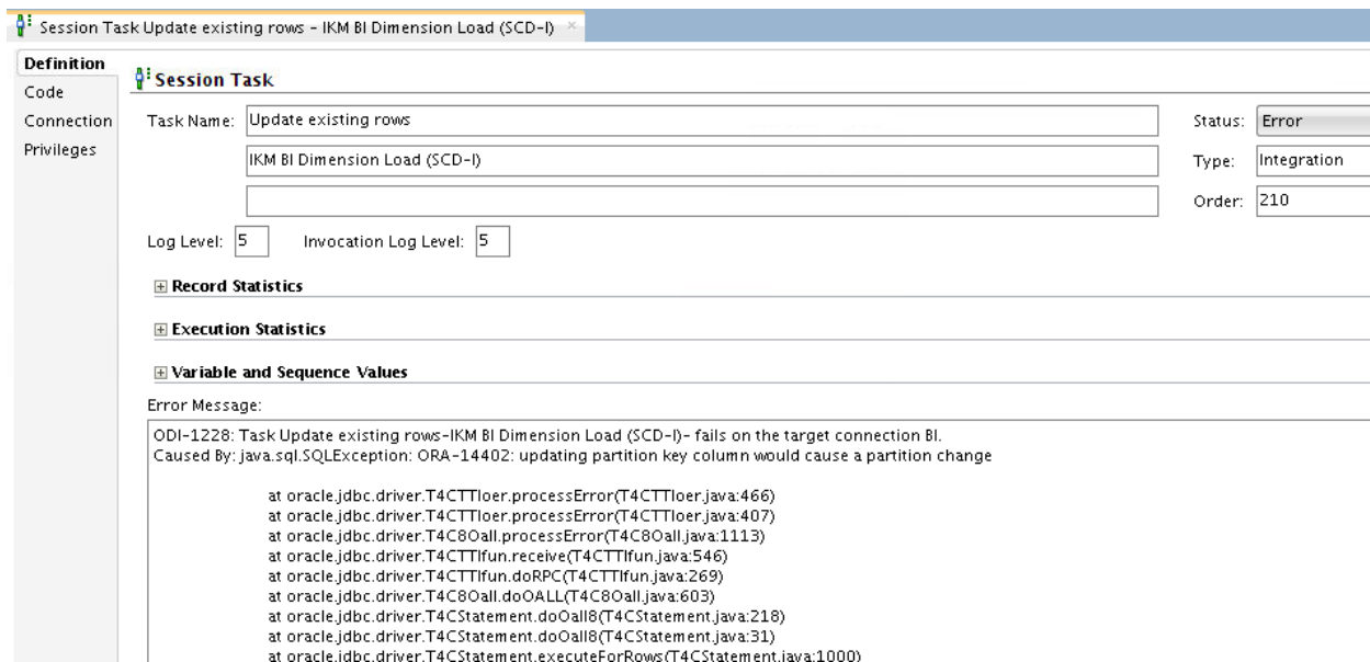
Figure 26: Viewing Error Details in ODI
