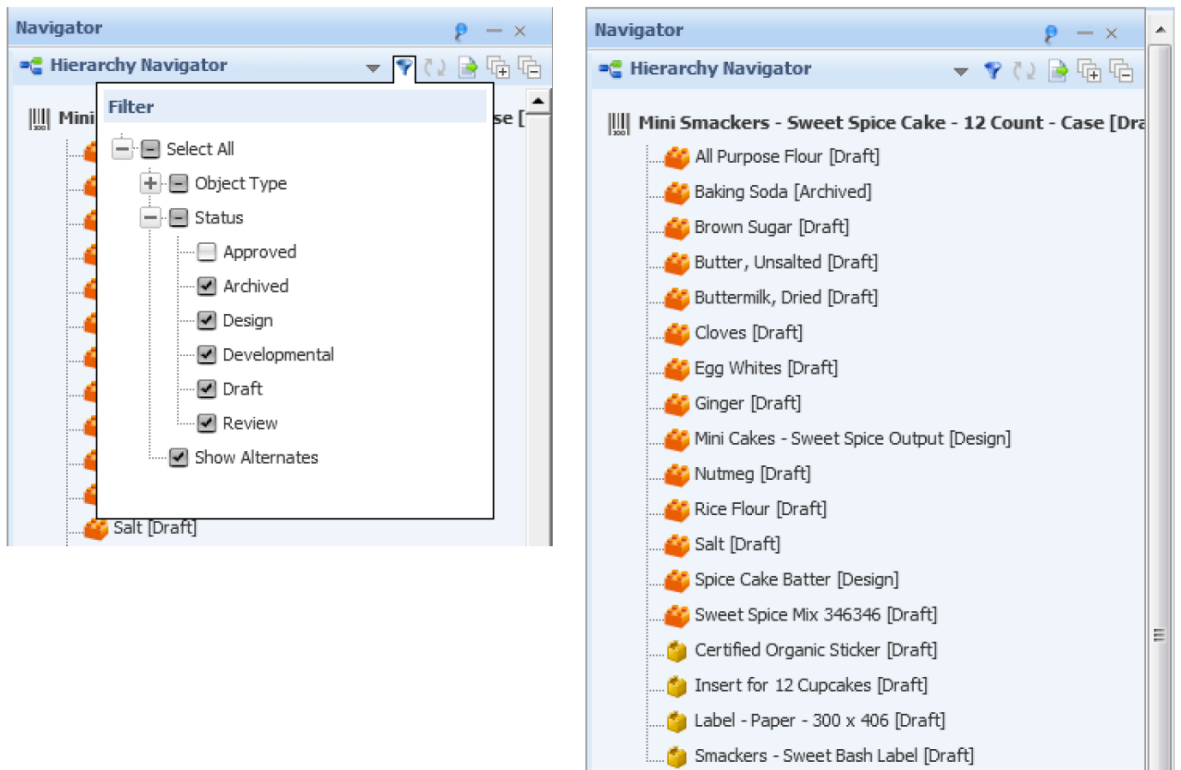
Figure 8. Quickly see all materials for a product hierarchy that aren't in an approved status
