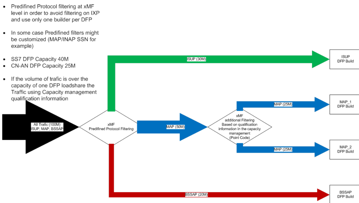
Figure 155: Final PMF Sigtran configuration Overview
