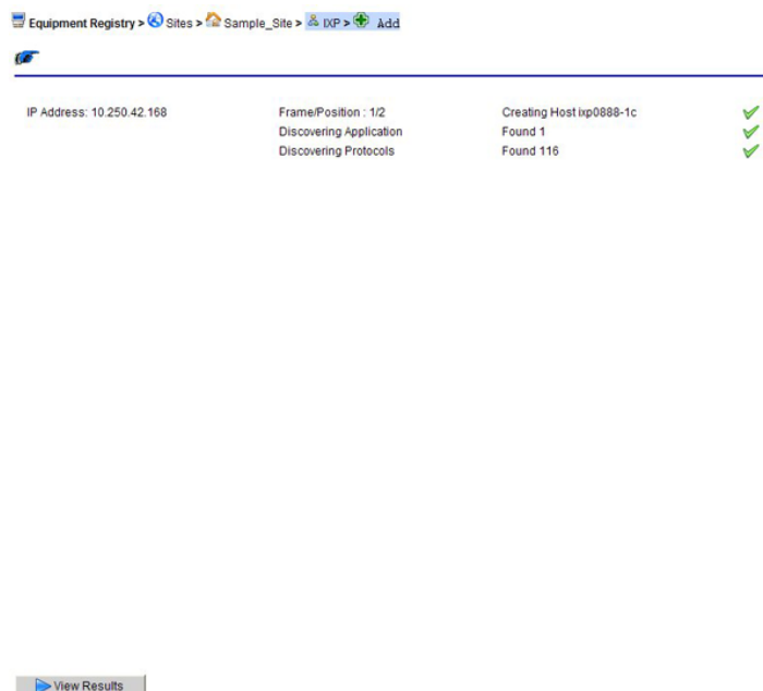
Figure 36: Subsystem Results Summary Screen
