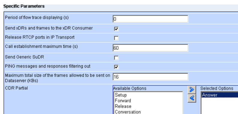
Figure 199: VoIP SIP with Answer selected
