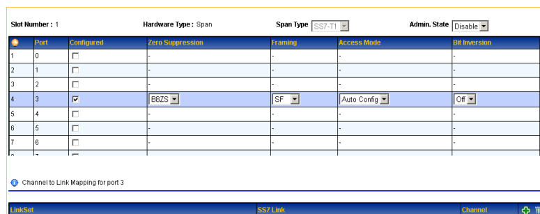
Figure 99: Span Card Configure Screen with Channel Link Mapping Section
