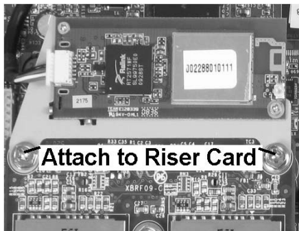
Figure 1: Installing the WiFi Card Bracket
