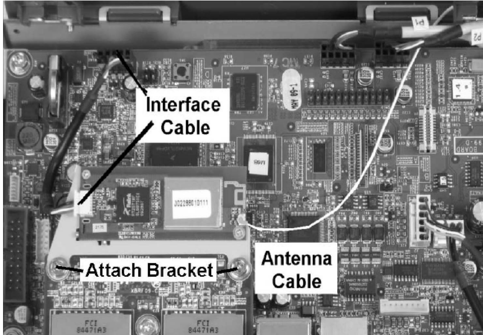
Figure 3: Installing the Bracket and Cables
