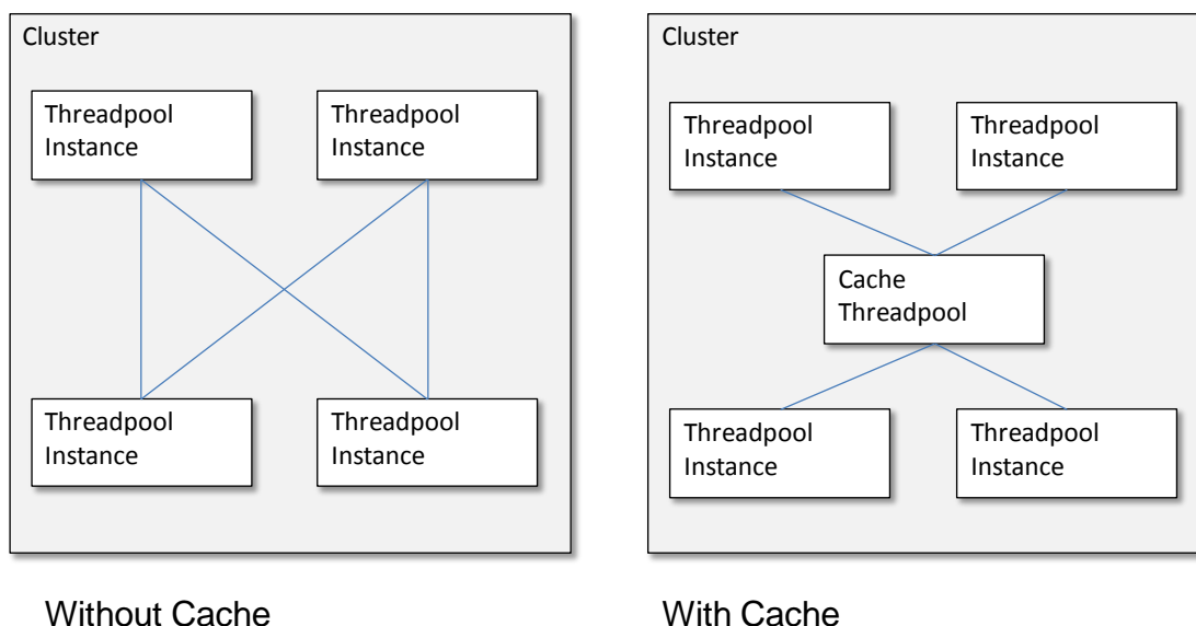
Figure 43 – Cache Architecture
