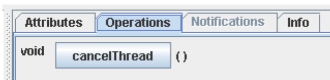
Figure 53 – Example cancelThread
