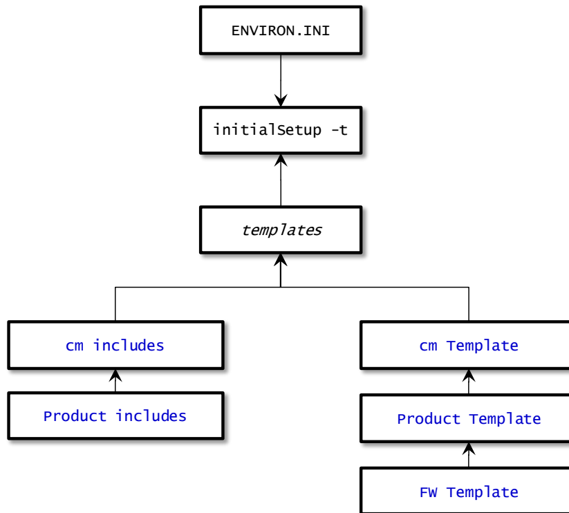
Figure 47 – Template Hierarchy
