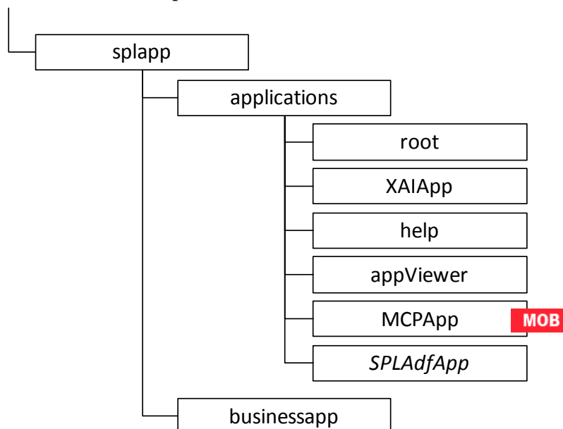
Figure 45 – Expanded Format
