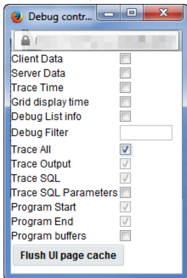
Figure 16 – Debug controls
