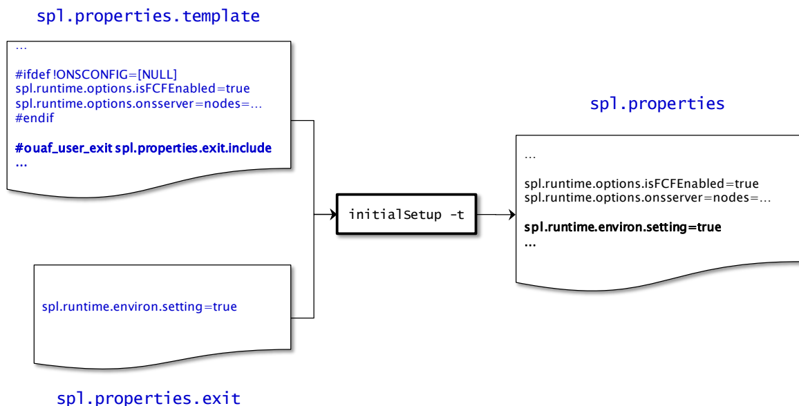
Figure 46 – Include files
