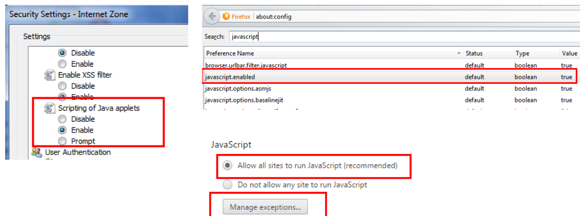
Figure 26 – Javascript Settings
