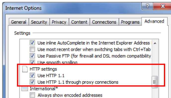
Figure 25 – HTTP 1.1 Settings
