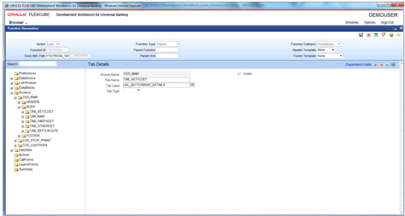
Fig 9.7 Tab Properties
