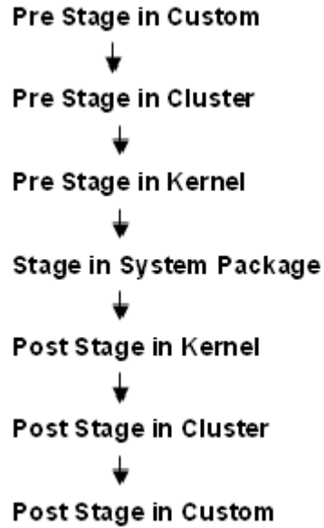
Fig 12.31: Flow of control through Hook Packages
