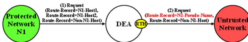
Figure 18: Route-Record Hiding - Request Message
