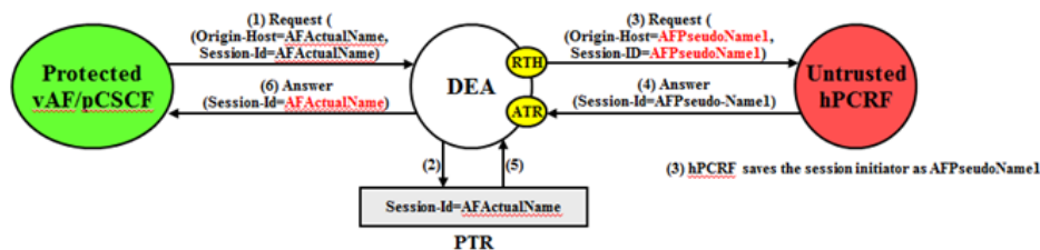
Figure 33: Protected vAF/pCSCF to Untrusted-hPCRF Transaction
