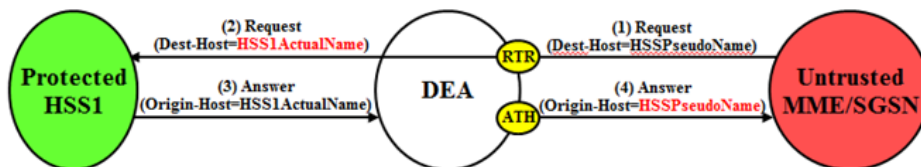
Figure 26: S6a/S6d HSS TH Untrusted-MME/SGSN to Protected-HSS Transaction
