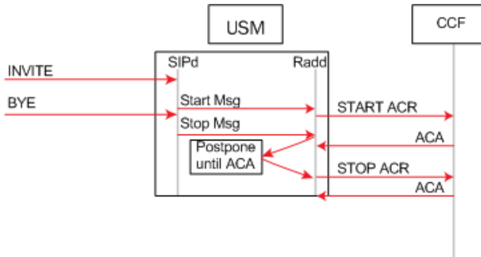
Call Flow Showing Delivery Postponement
