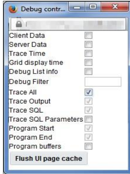
Figure 16: Debug Controls
