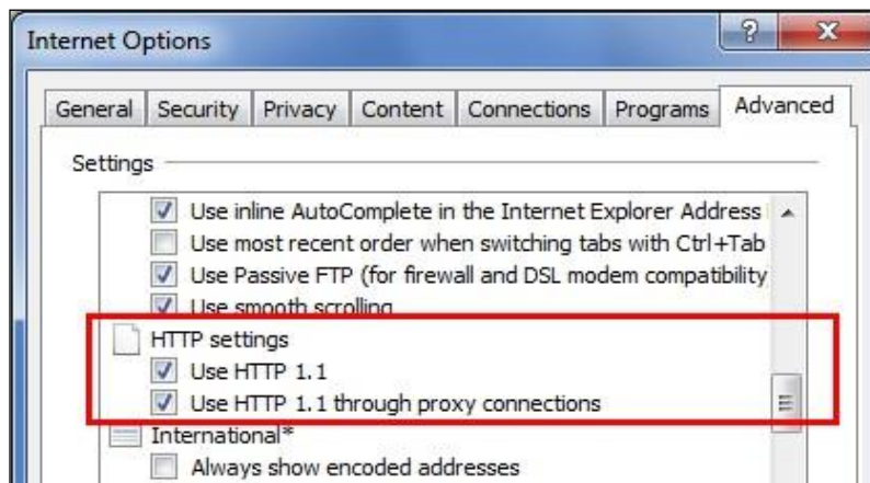
Figure 25: HTTP 1.1 Settings
