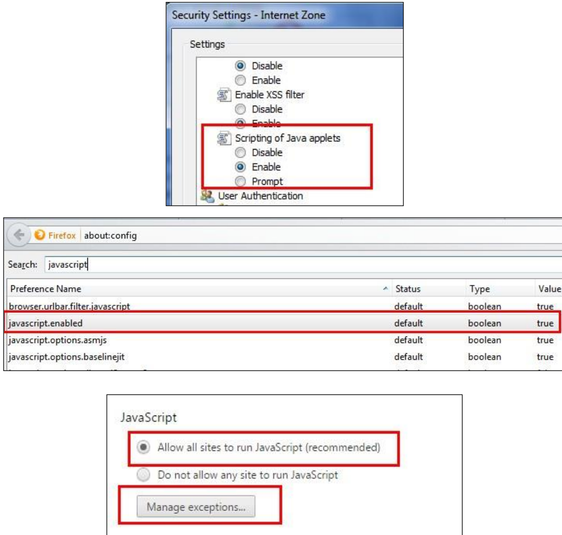
Figure 26: Javascript Settings
