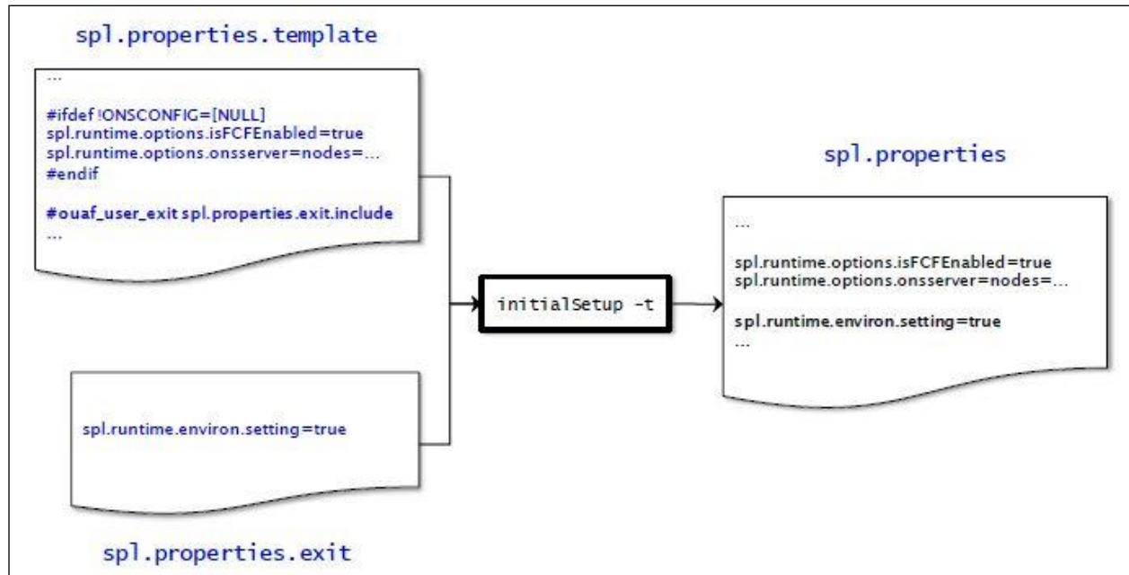
Figure 46: Include Files
