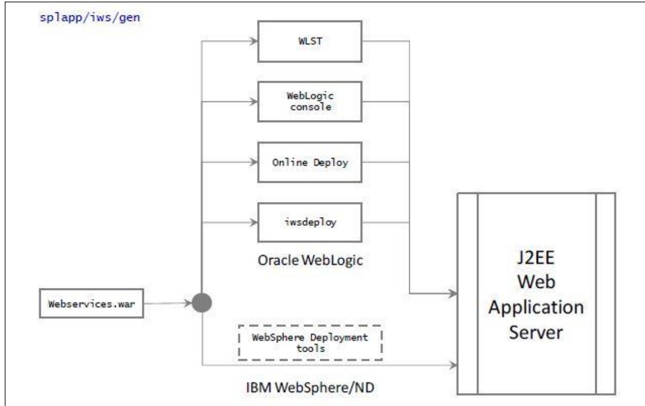
Figure 38: Inbound Web Services Deployment Process
