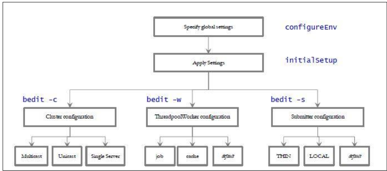
Figure 42: bedit Configuration Process
