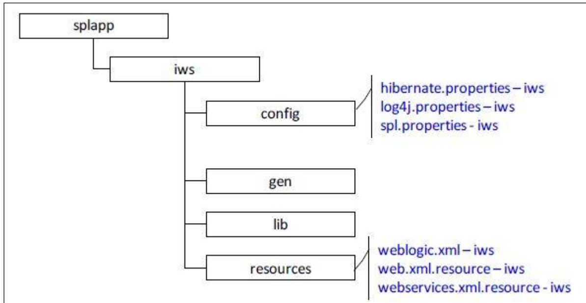
Figure 36: Inbound Web Services Structures
