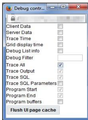
Figure 16: Debug Controls
