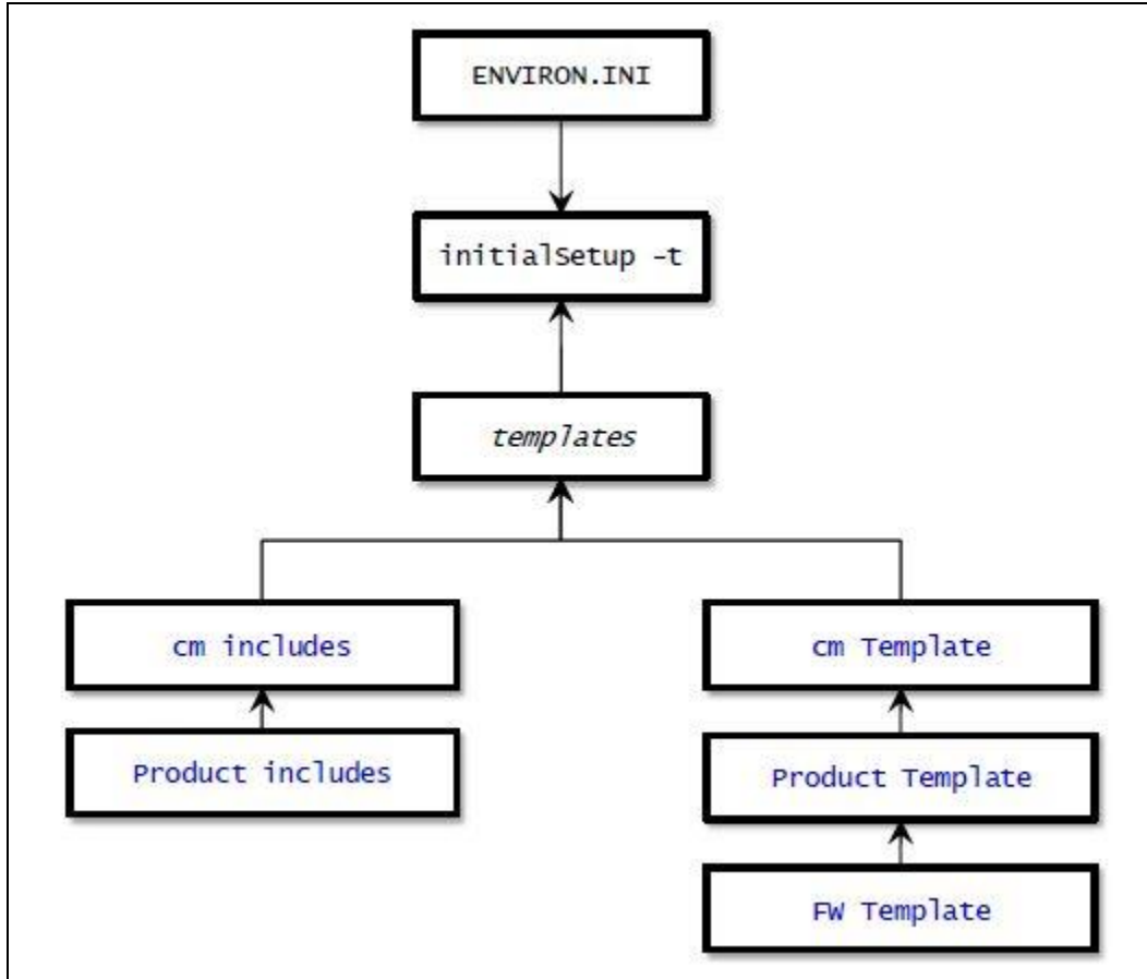
Figure 47: Template Hierarchy
