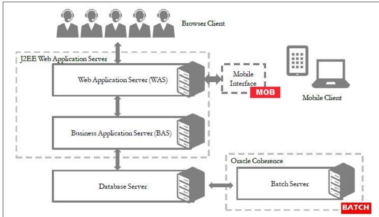
Figure 1: Product Architecture
