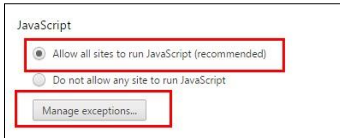
Figure 26: Javascript Settings
