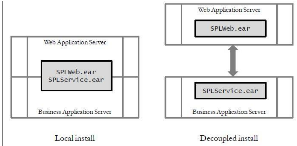
Figure 31: Installation Modes
