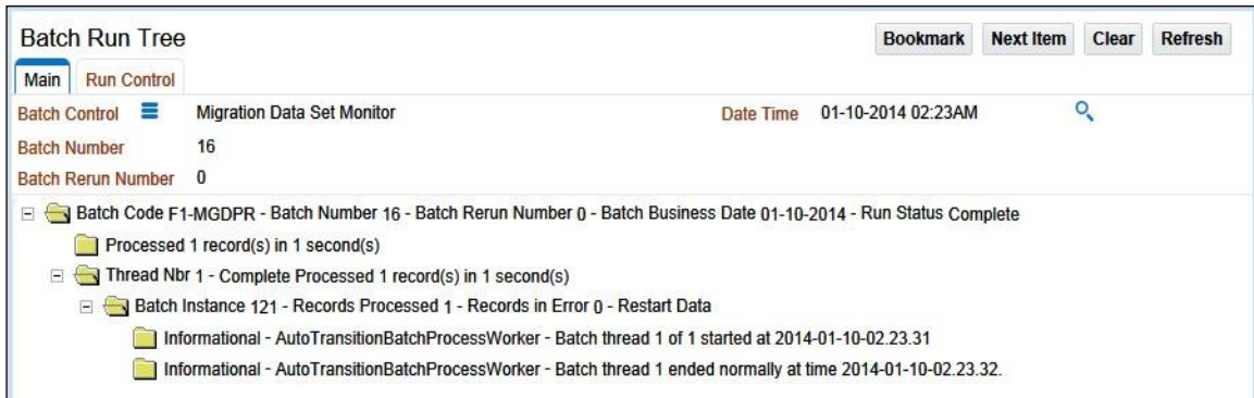
Figure 11: Batch Run Execution Example
