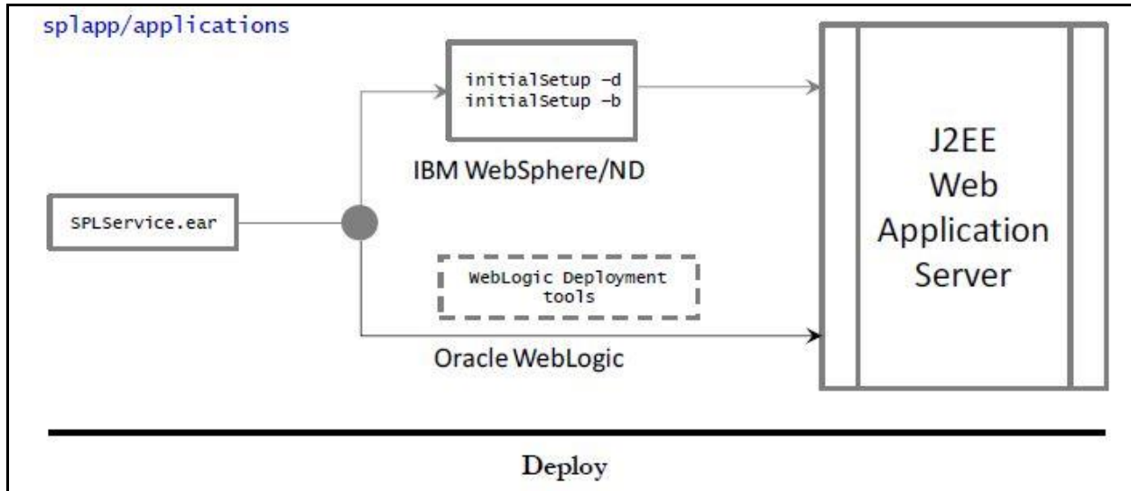
Figure 34: Business Application Server Deployment Process
