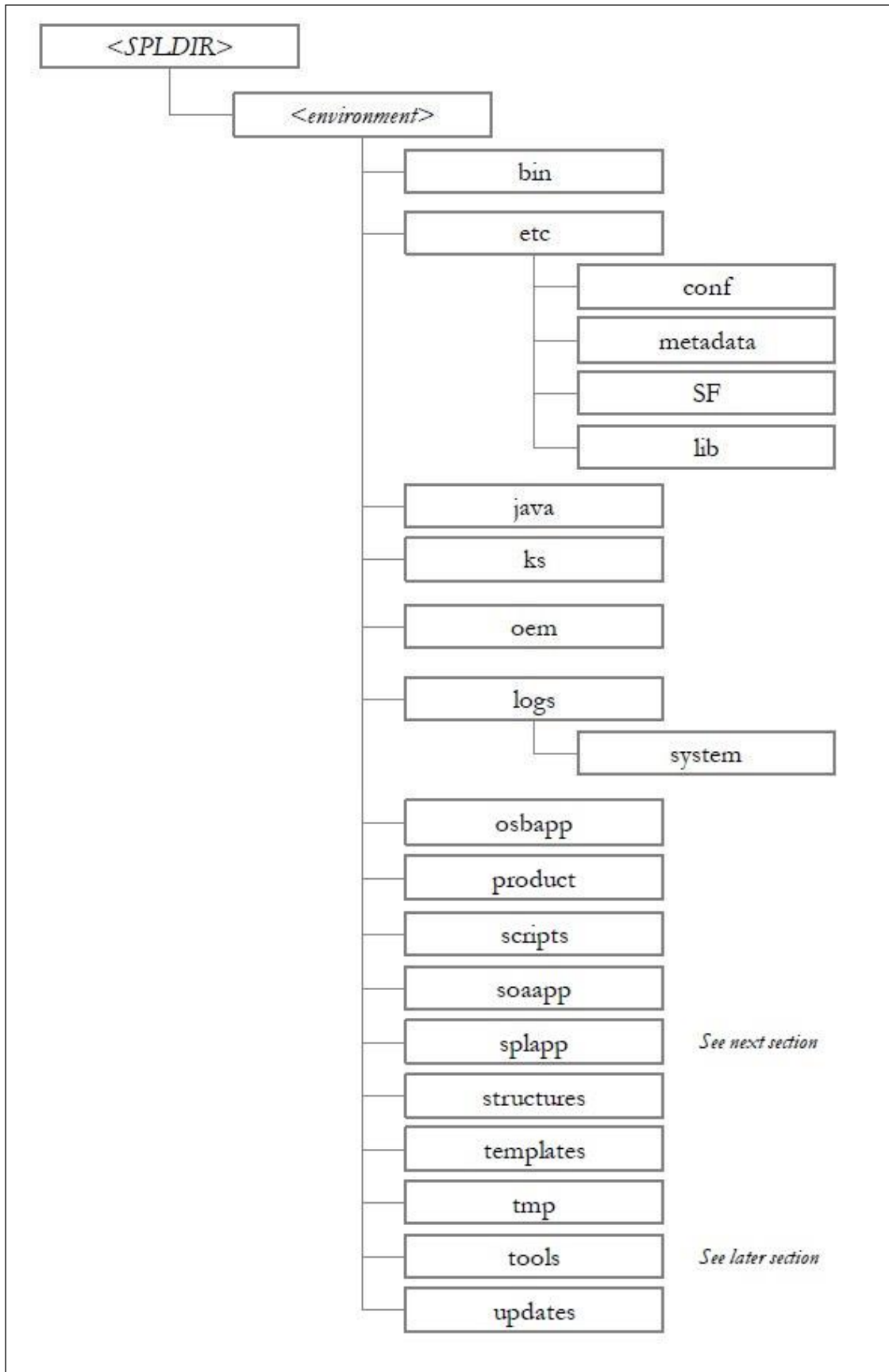
Figure 5: Software Directory Structure
