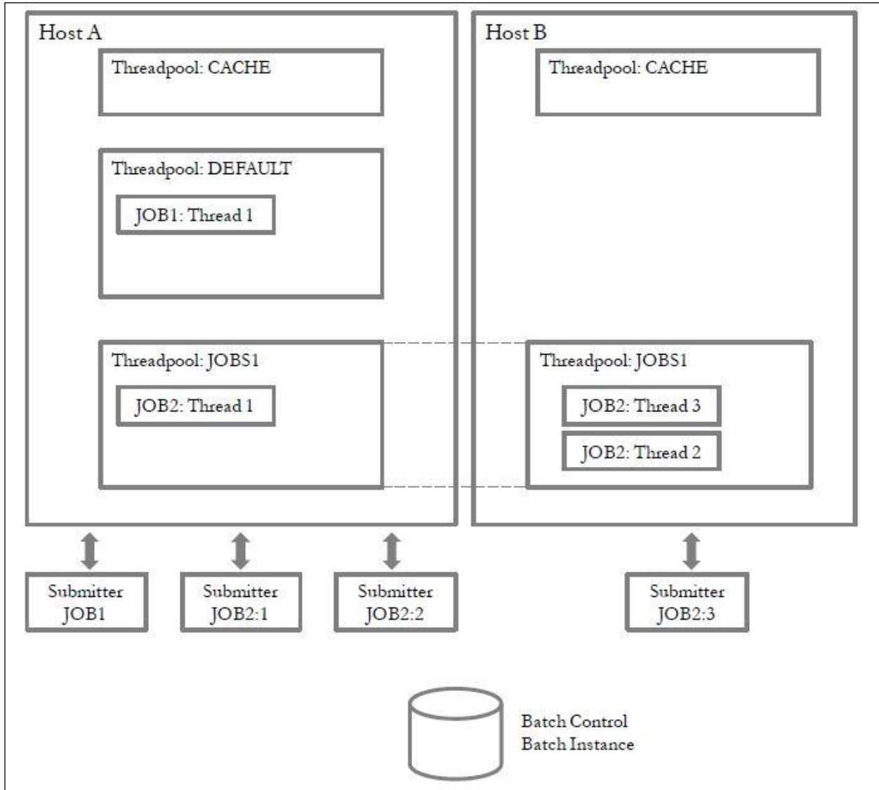
Figure 3: Batch Architecture Overview
