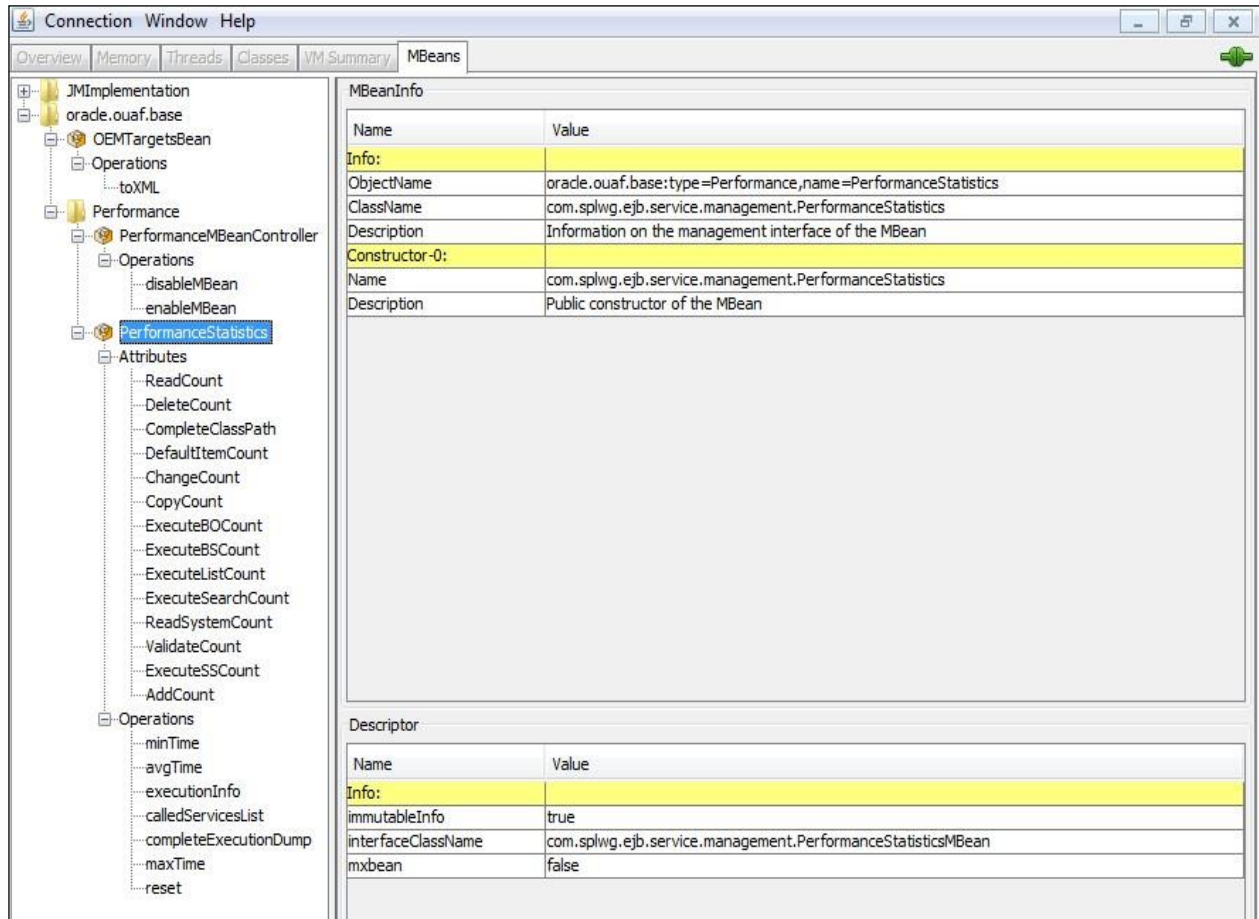
Figure 19: Business Application Server Mbeans in jconsole Example
