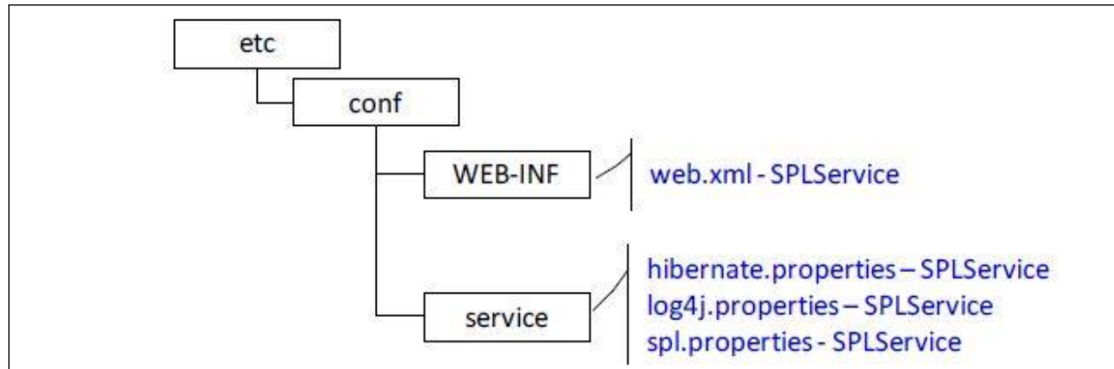
Figure 33: Business Application Server Configuration Files
