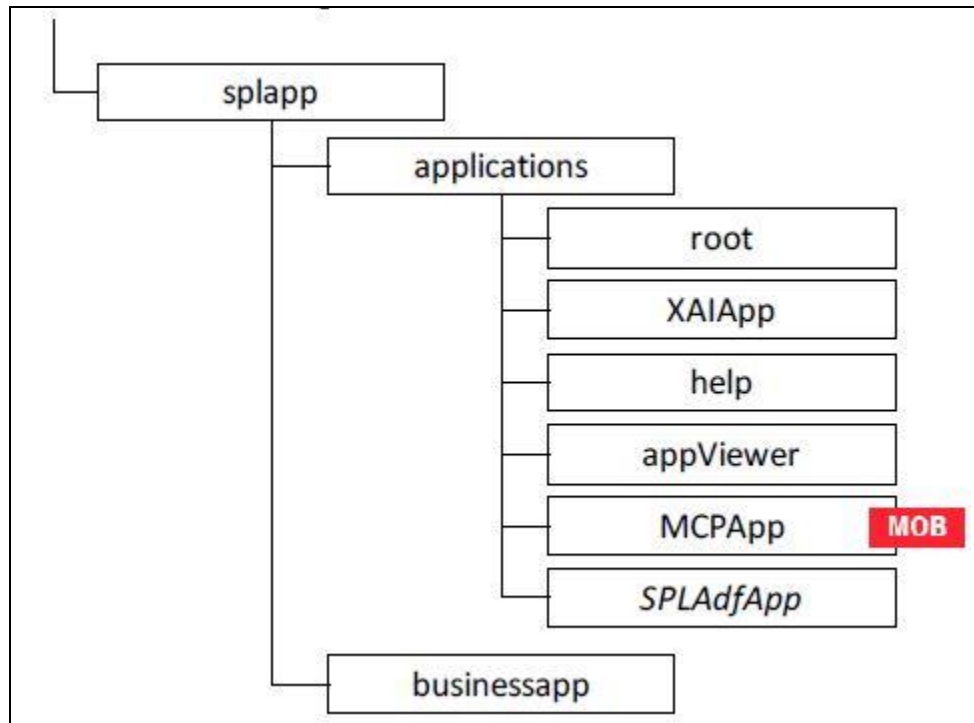
Figure 45: Expanded Format
