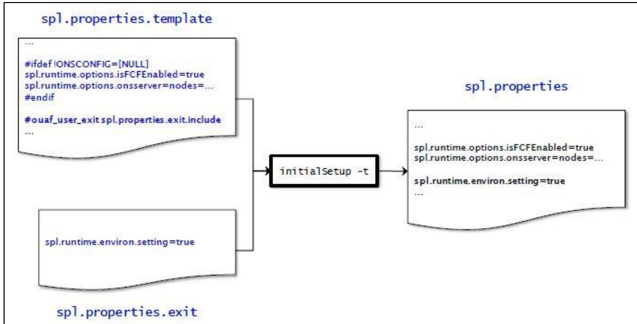
Figure 46: Include Files
