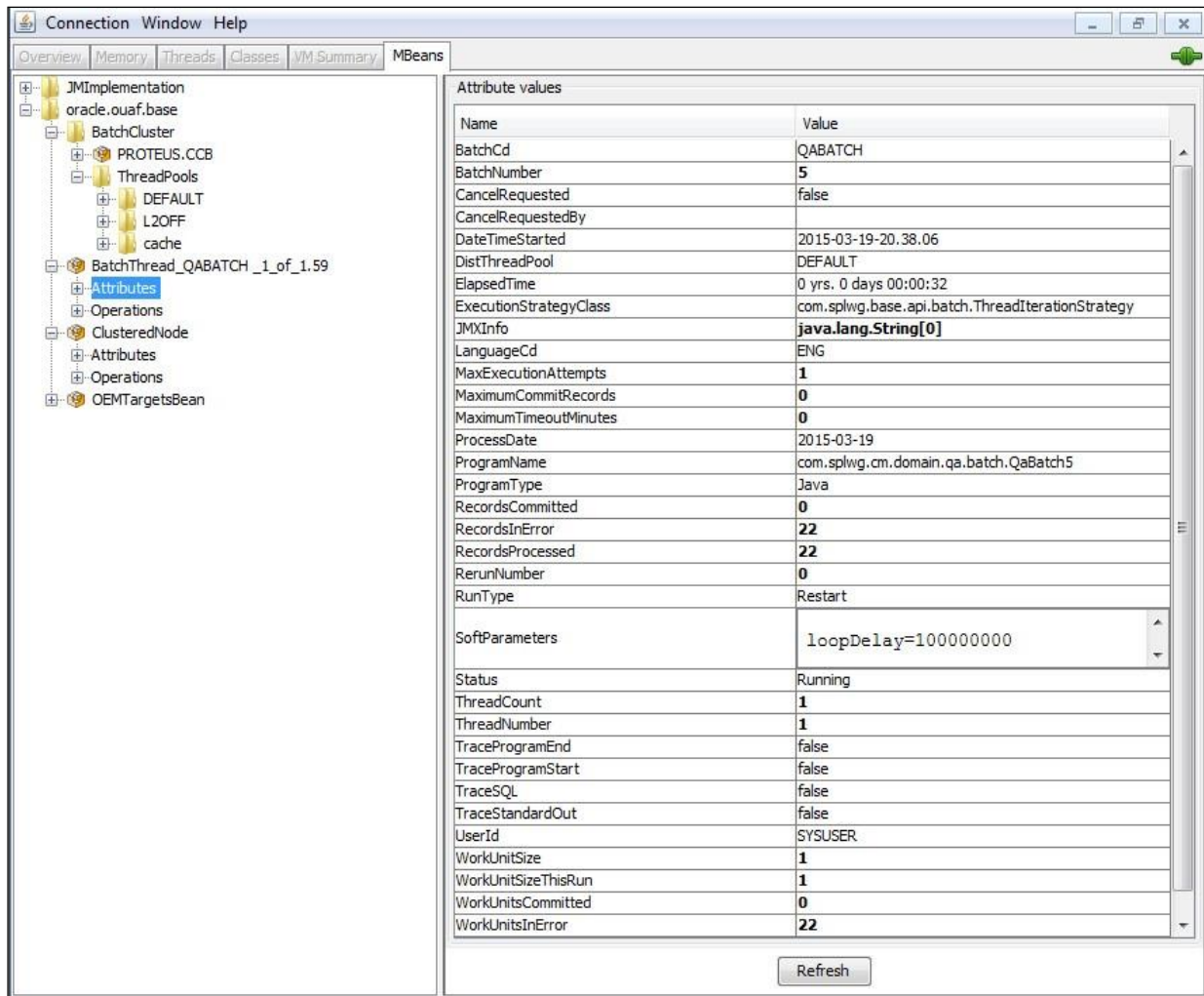
Figure 22: Batch Thread Mbean in jconsole Example
