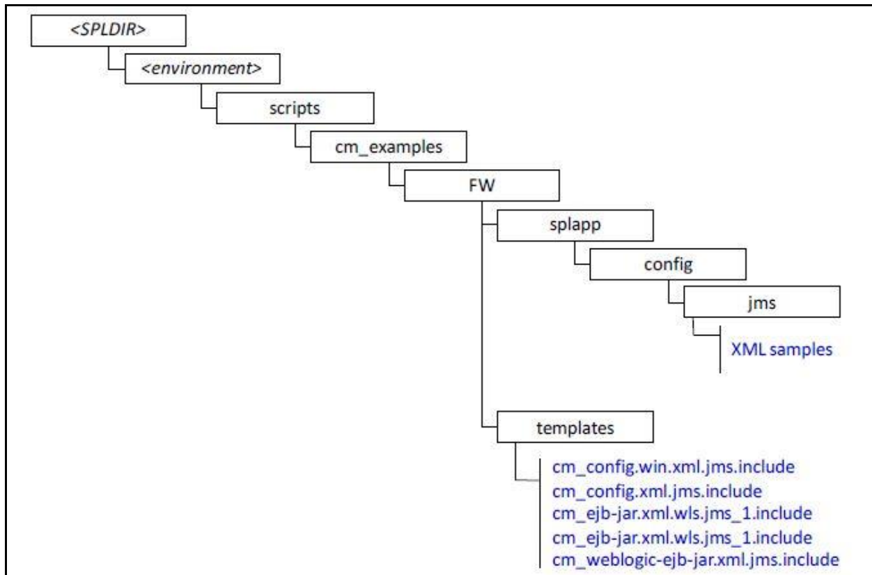
Figure 48: Custom JMS Configuration
