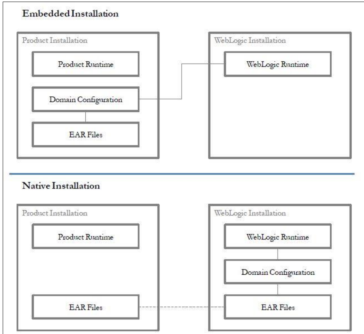
Figure 4: Native and Embedded Architectures
