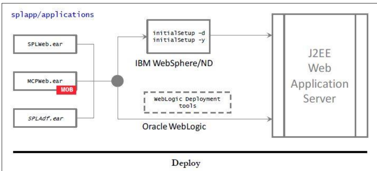
Figure 30: Web Application Server Deployment Process
