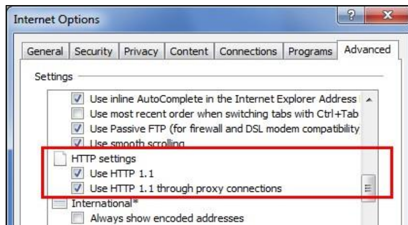
Figure 25: HTTP 1.1 Settings
