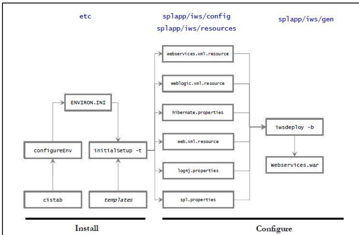
Figure 37: Inbound Web Services Configuration Process
