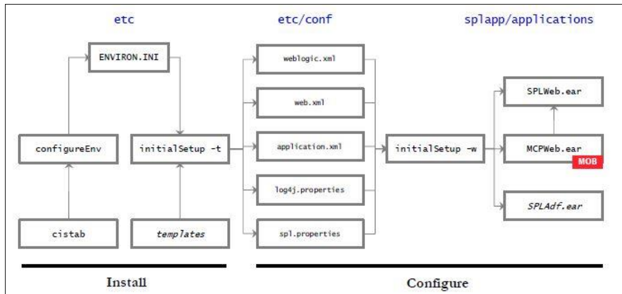
Figure 29: Web Application Server Configuration Process
