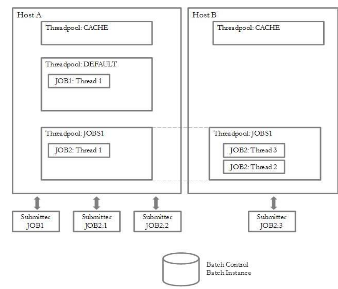
Figure 3: Batch Architecture Overview
