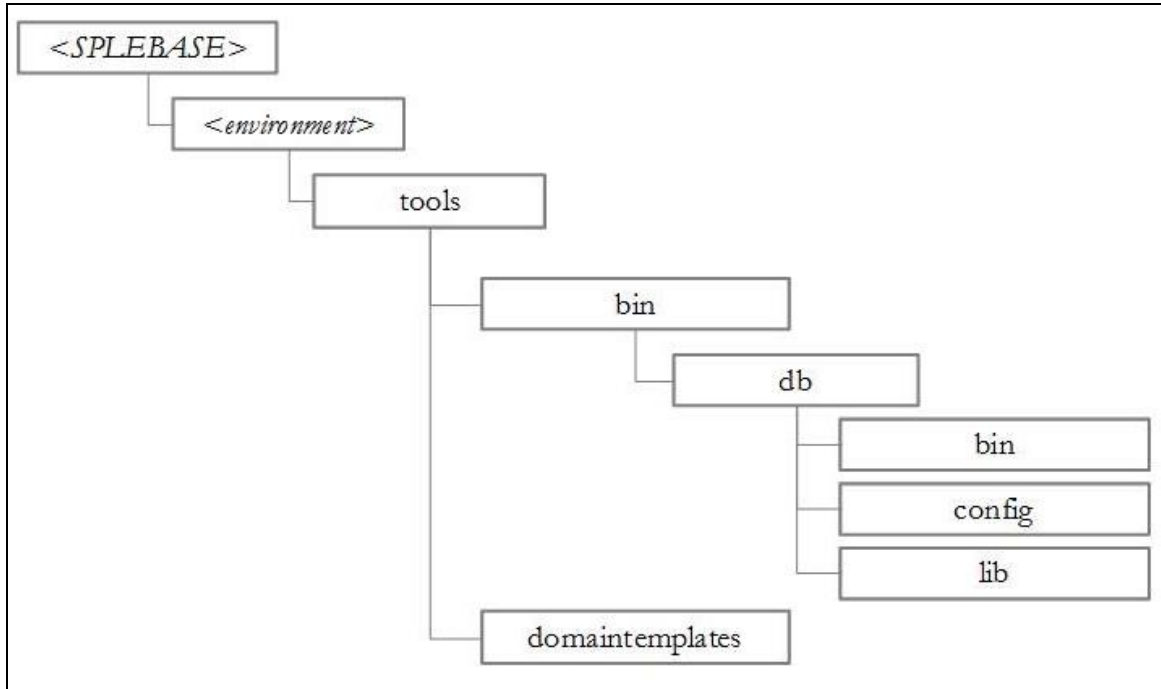
Figure 7: Tools Directory Structure
