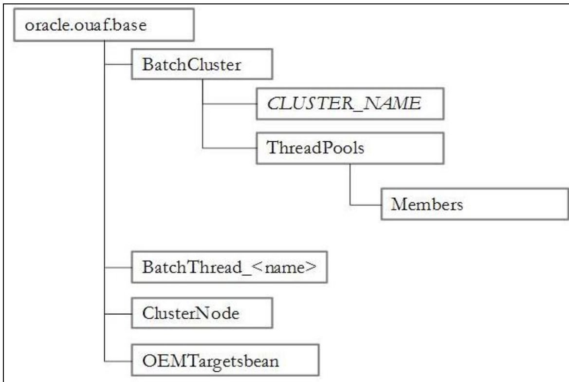
Figure 18: Batch Server Mbeans
