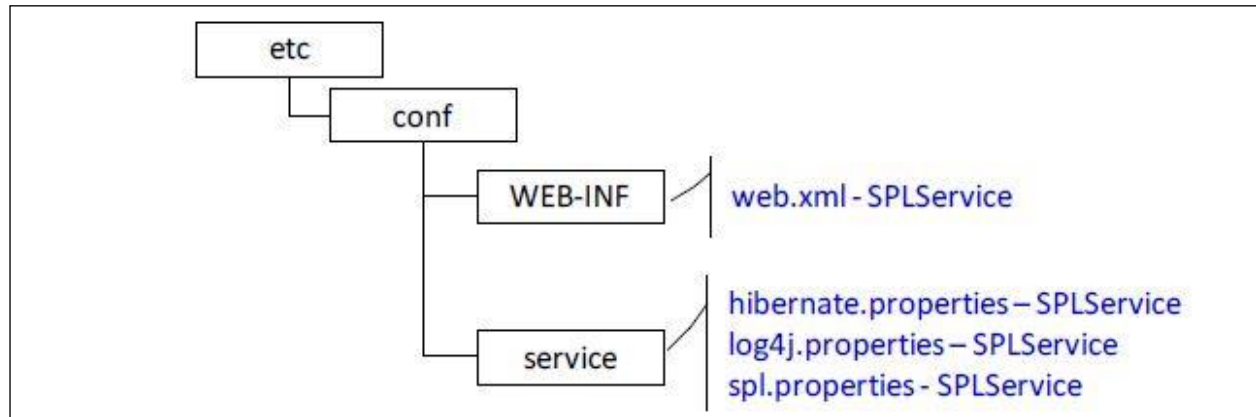
Figure 27: Business Application Server Configuration Files
