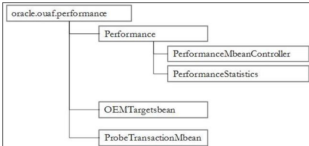
Figure 15: Business Application Server Mbeans
