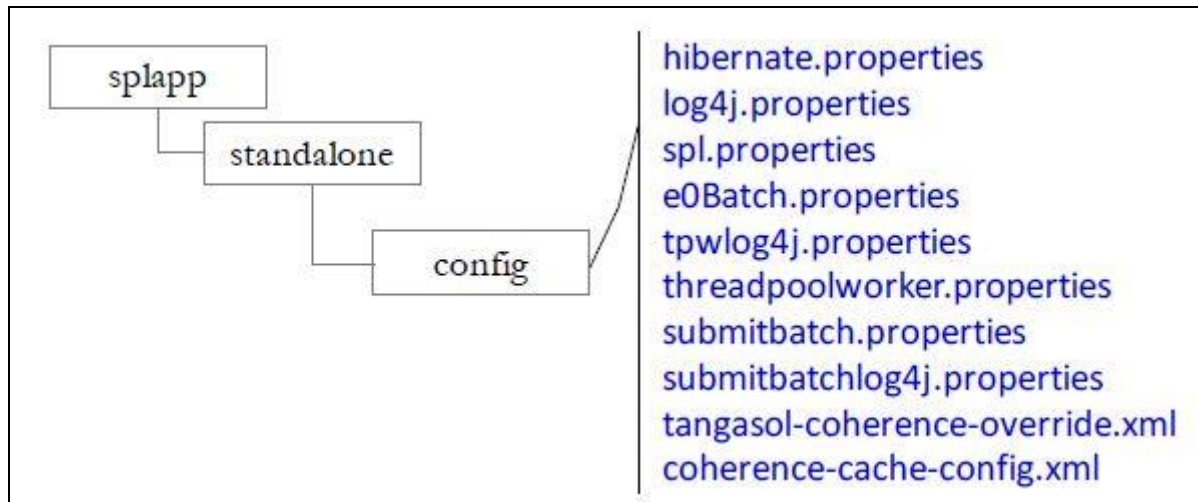
Figure 34: Batch Configuration Files
