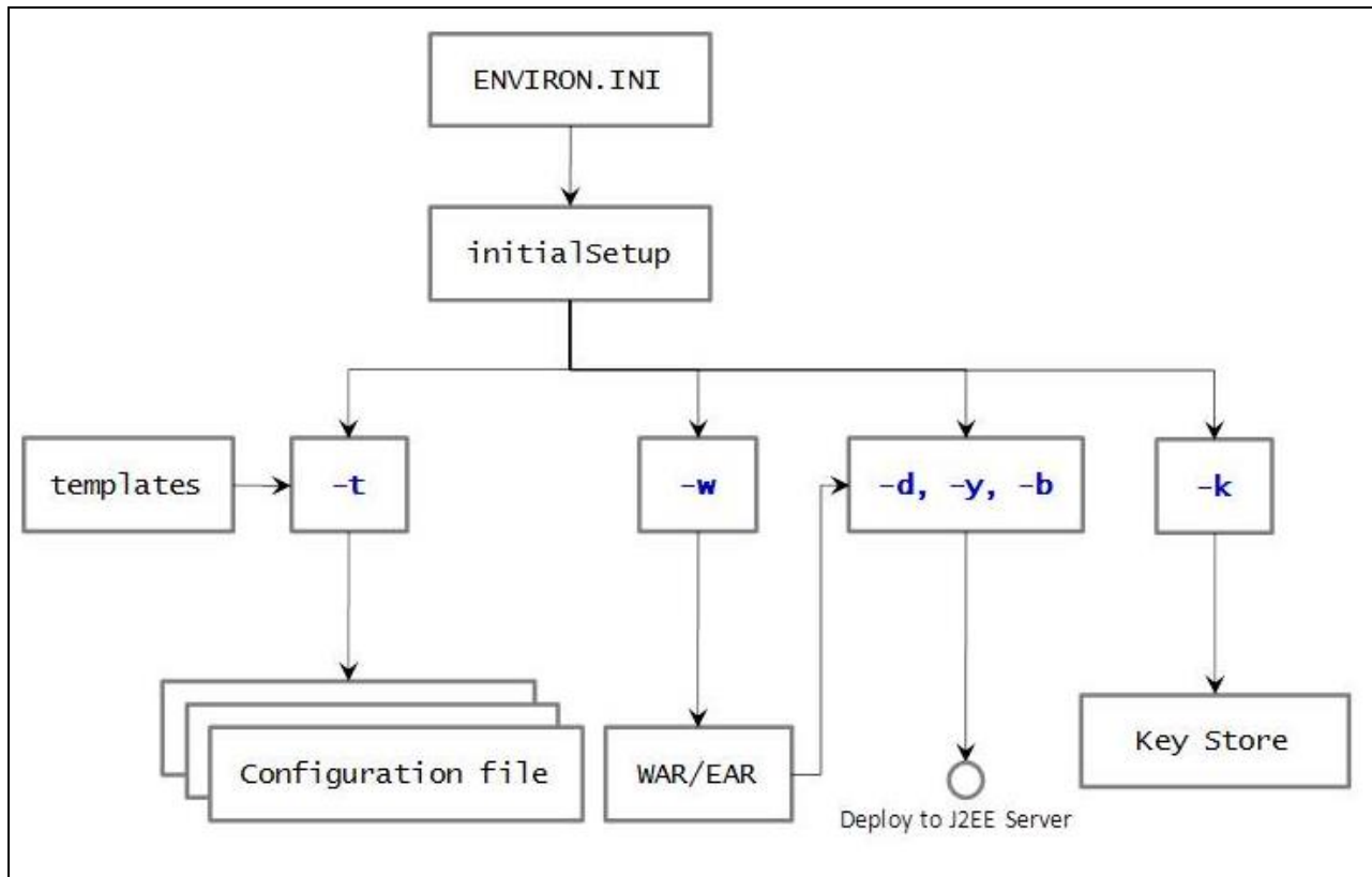
Figure 9: initialSetup Command Structure
