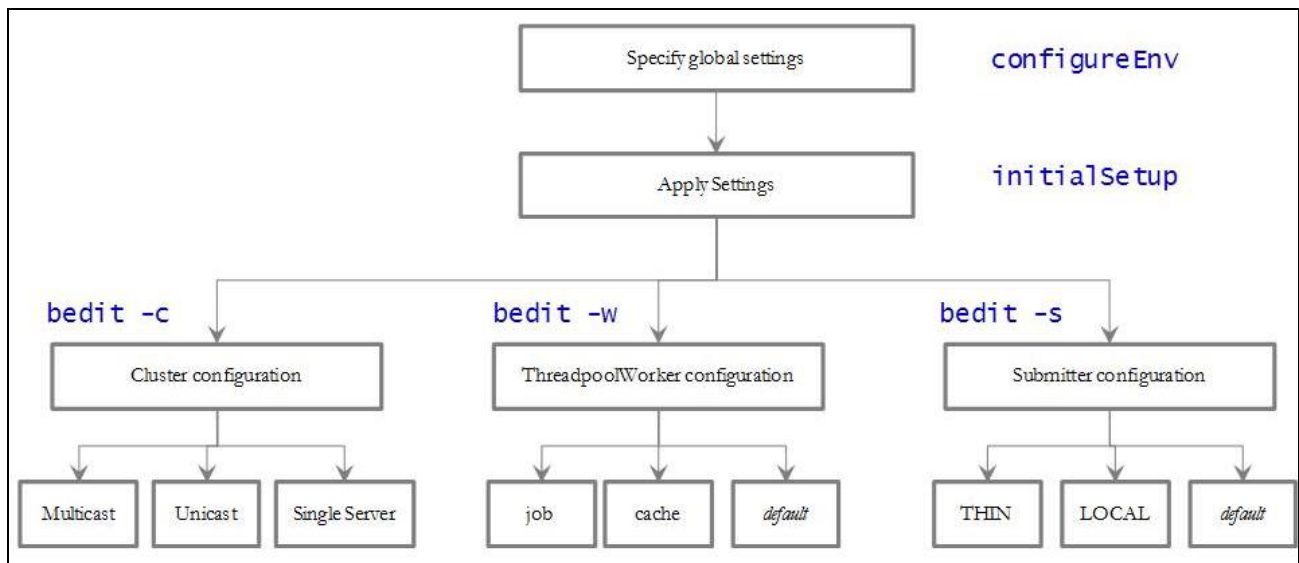
Figure 36: bedit Configuration Process
