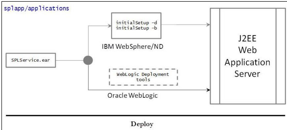
Figure 28: Business Application Server Deployment Process
