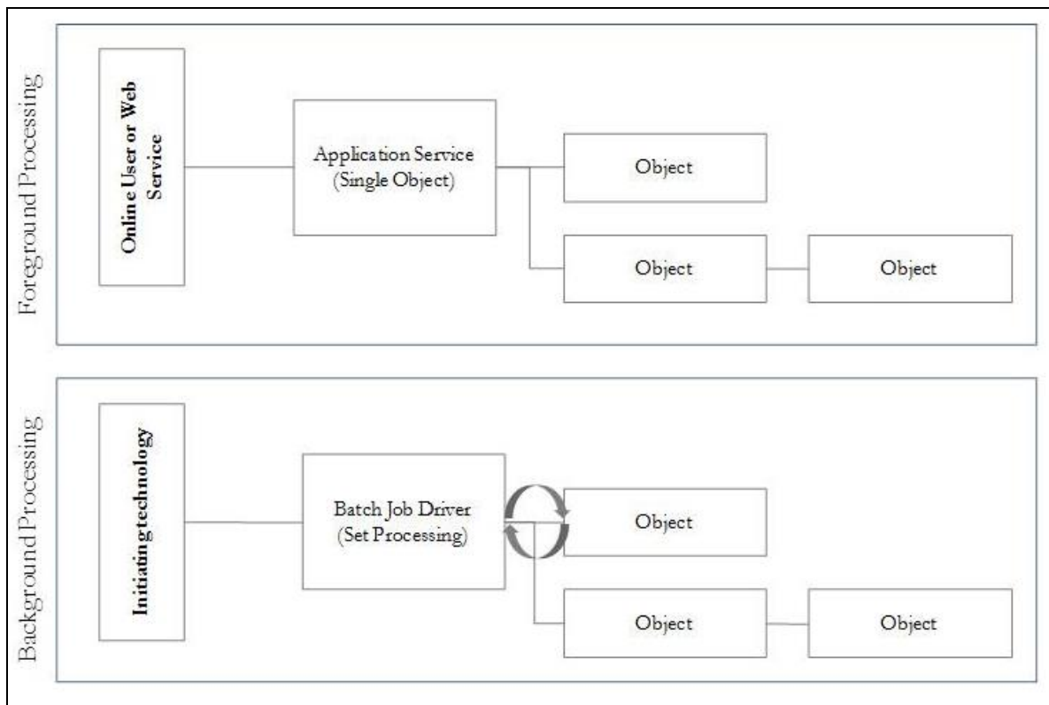
Figure 2: Batch Processing Architecture
