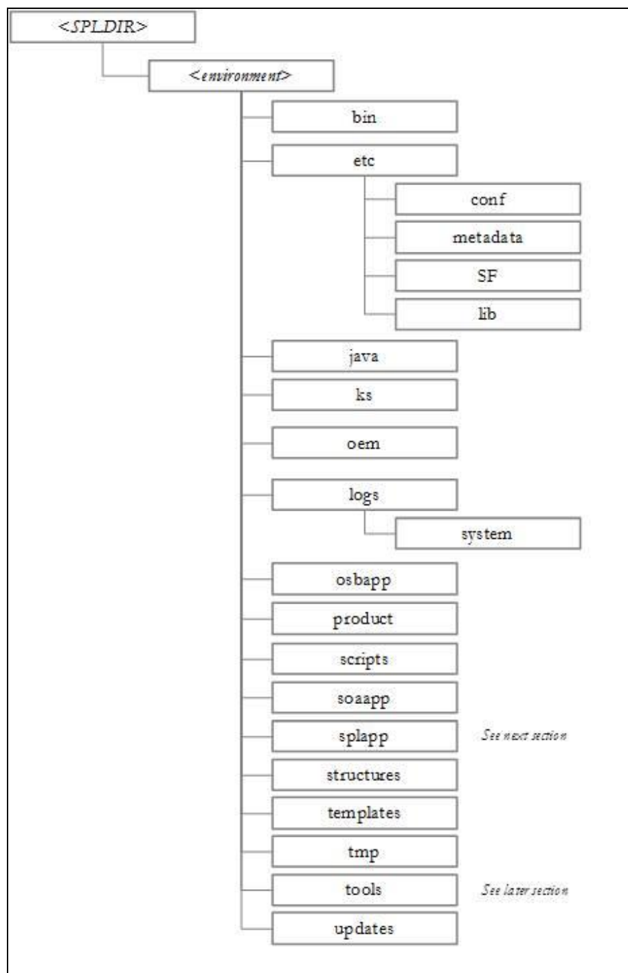
Figure 5: Software Directory Structure
