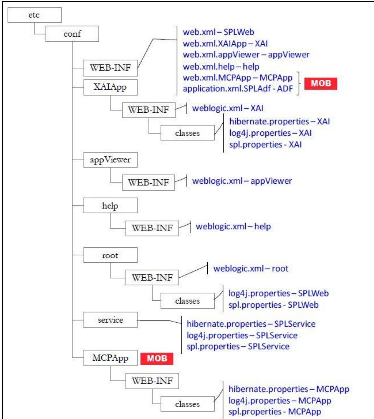
Figure 22: Configuration File Hierarchy
