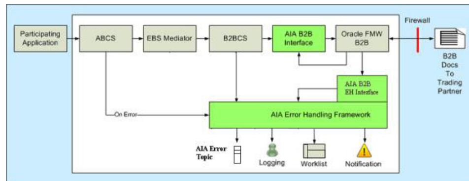
Figure 20–4 Foundation Pack B2B Infrastructure Components
