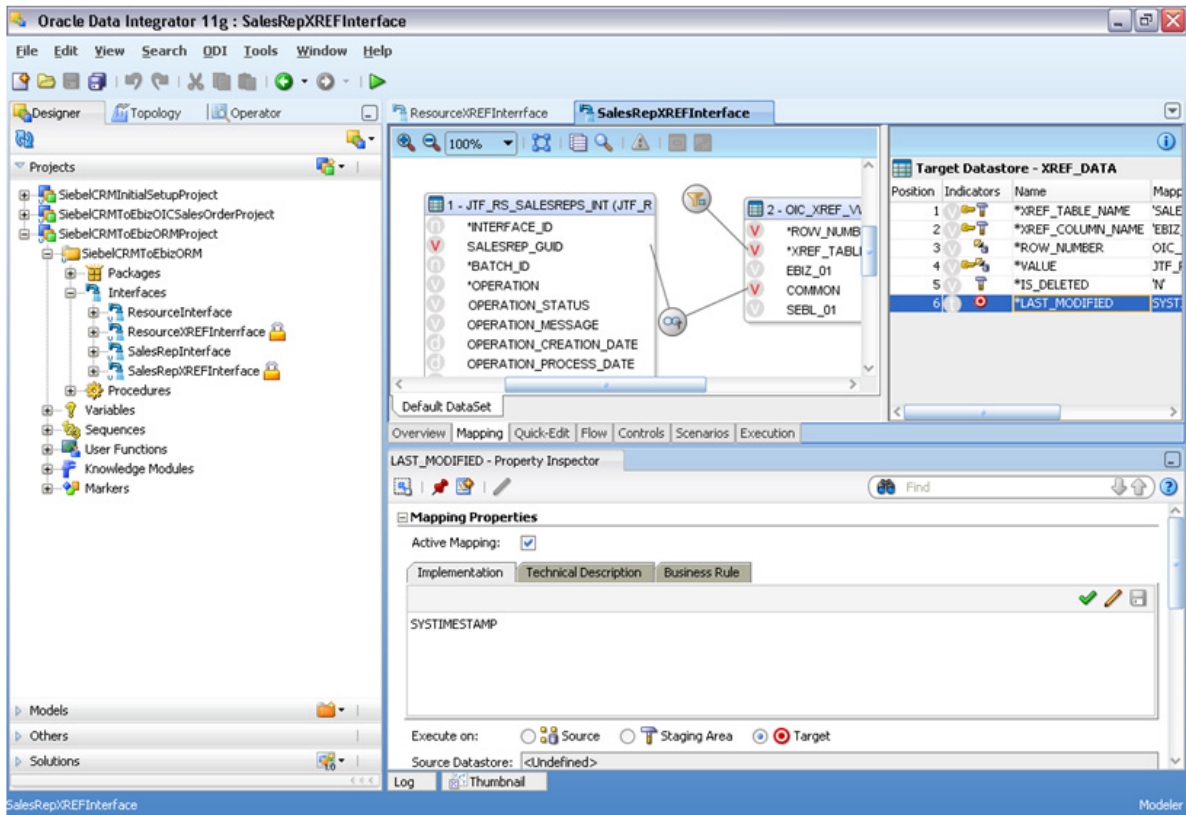
Figure 16–15 Implementation Tab Value Set to SYSTIMESTAMP
