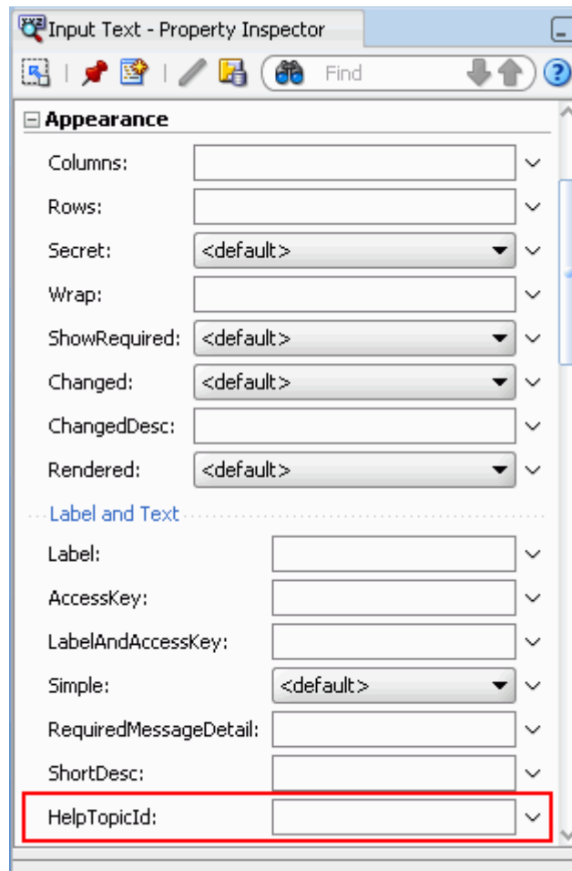
Figure 20–2 HelpTopicId Attribute
