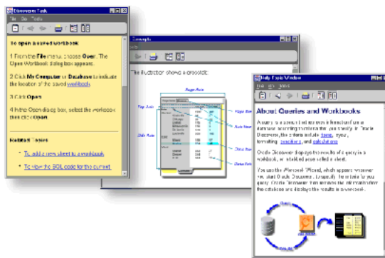
Figure 2-3 Topic Windows
