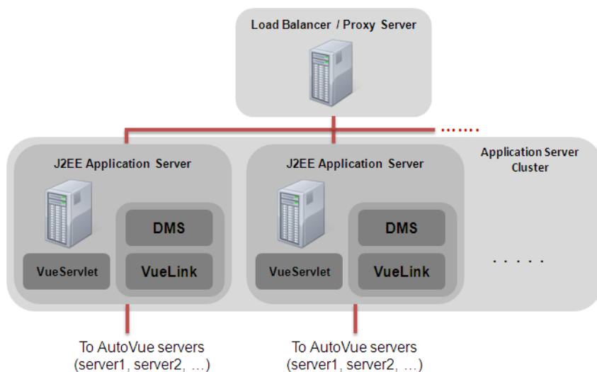
Figure 4-4 VueServlet Cluster
