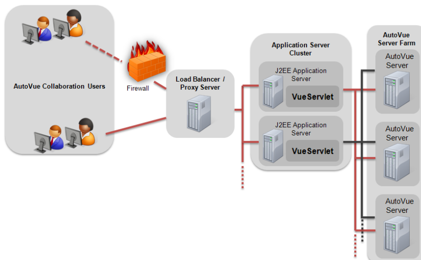
Figure 5-1 RTC Deployment
