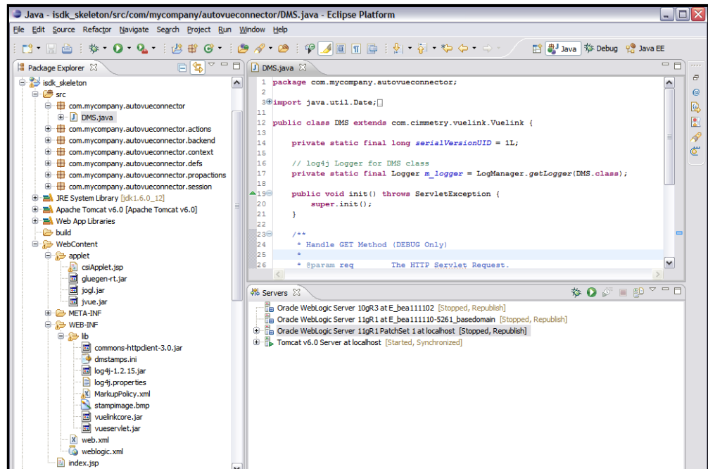
Figure 3 Eclipse workspace
