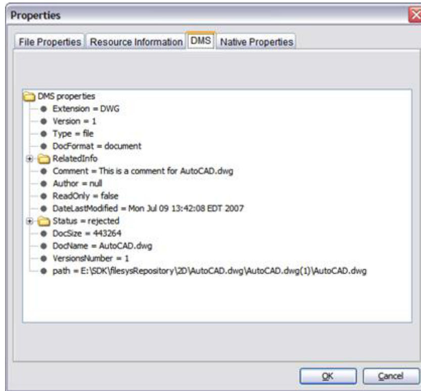
Figure 6–3 Properties dialog
