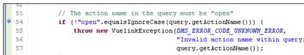
Figure 5-1 Set breakpoint
