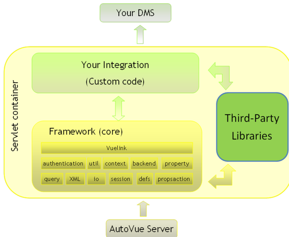
Figure 4–1 Your Integration
