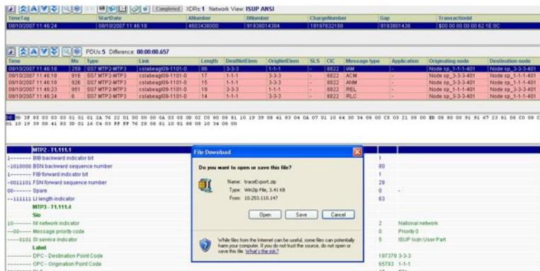
Figure 52: Export Screen
