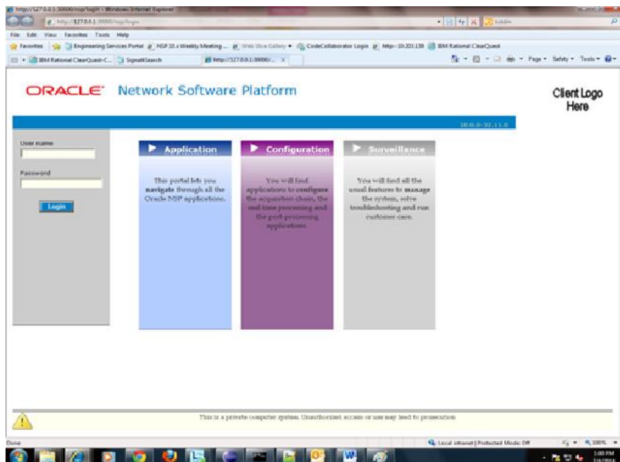
Figure 10: NSP Portal
