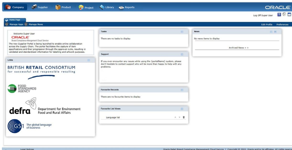
Figure 2–6 Home Page
