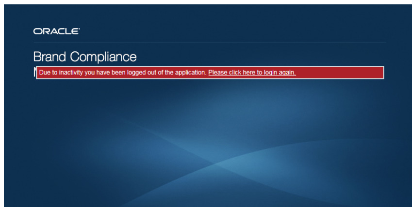
Figure 2–12 Session Expired
