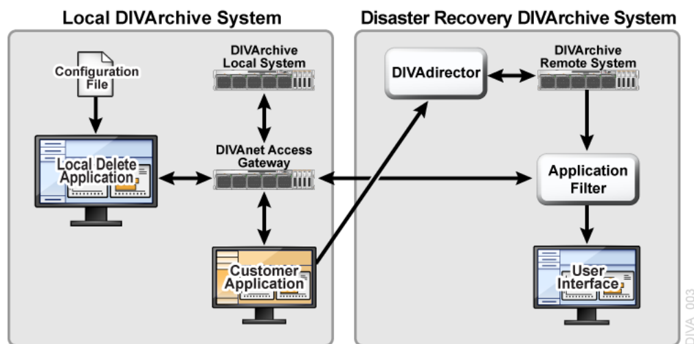
Figure 1-1 Standard Local Delete Workflow
