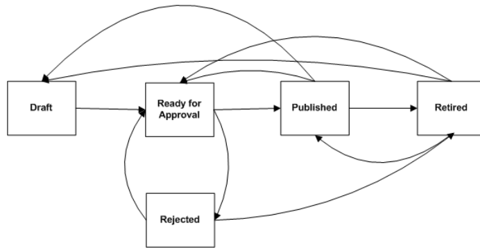
Figure 5–1 Default Content Workflow Diagram
