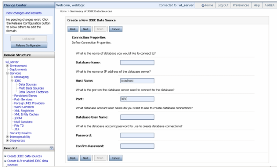
Figure 3–4 Create a New JDBC Data Source—JDBC Data Source Connection Properties Page
