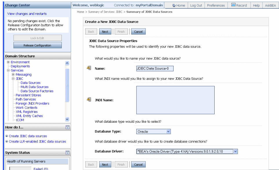
Figure 3–3 Create a New JDBC Data Source—JDBC Data Source Properties Page
