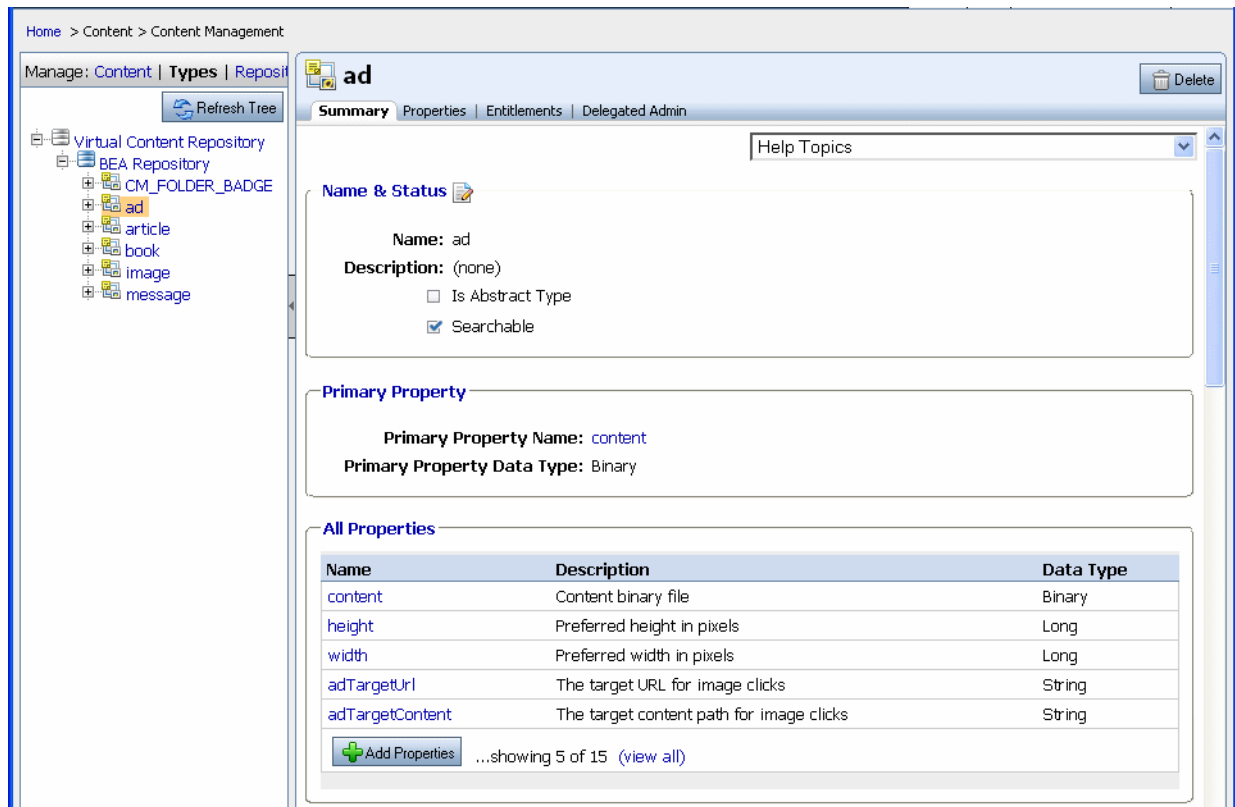
Figure 6–5 The Types Tab within the Manage Types Window
